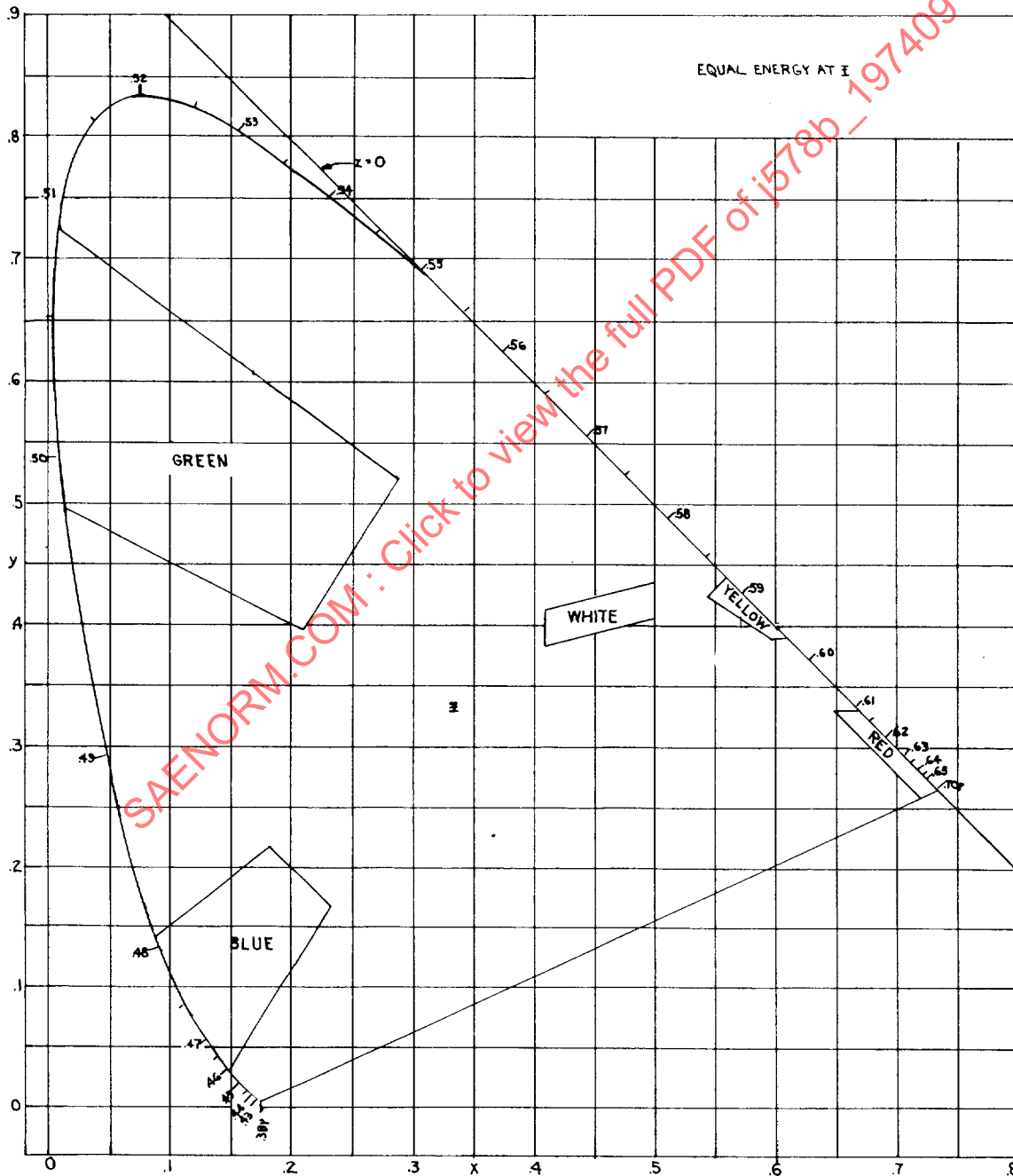
FIG. 1—CIE CHROMATICITY DIAGRAM
