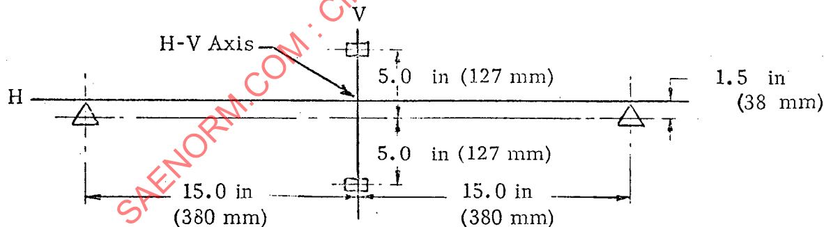
FIG. 1—TEST POINTS ON SCREEN AT 25 FT (7.6 m)
