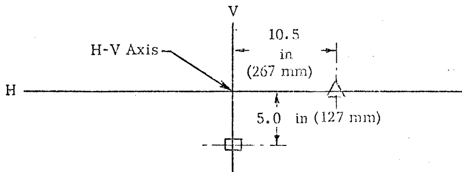
FIG. 2—TEST POINTS ON SCREEN AT 25 FT (7.6 m)
