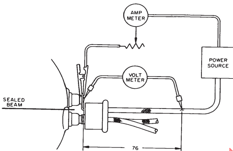
FIG. 1 - CONNECTOR TEST
