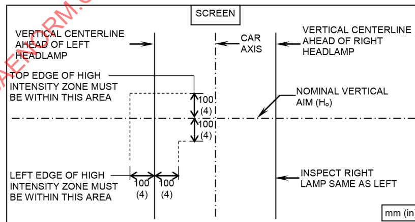
Figure 3 - Aim inspection limits for low beam headlamps which are not VOR or VOL
