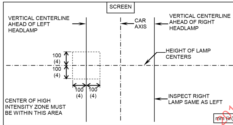
Figure 6 - Aim inspection limits for high beam headlamps
