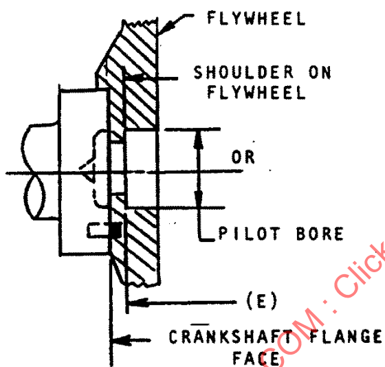
1 3B—When Pilot Bore Shoulder is located on the Flywheel
