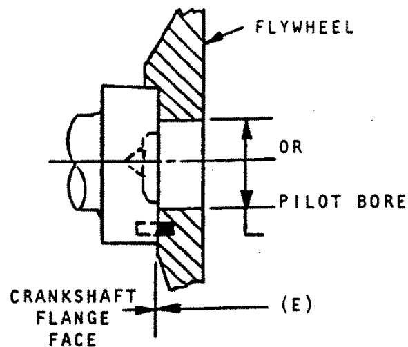
1 3A—When Pilot Bore Stop Face is Located at Crankshaft Flange Face
