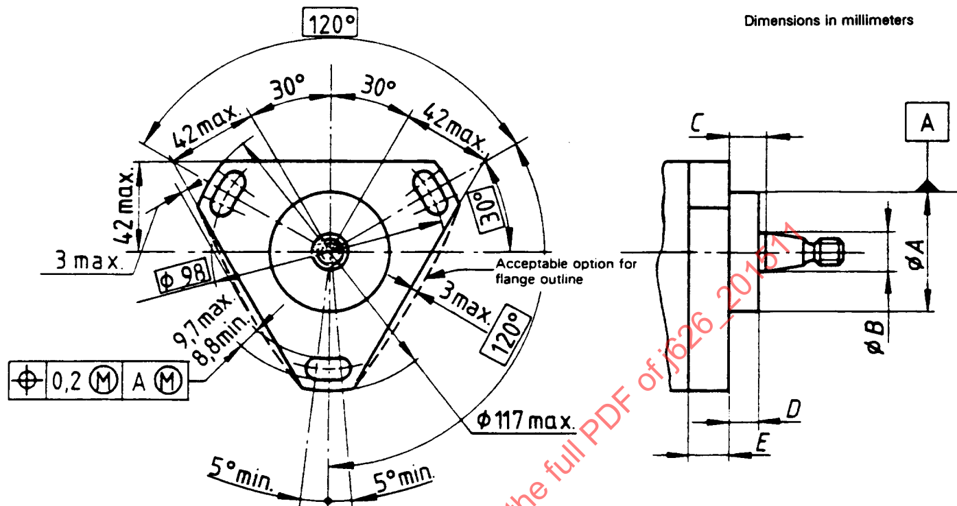
FIGURE 2—FUEL INJECTION PUMPS—TYPE 2 END-MOUNTING FLANGE
