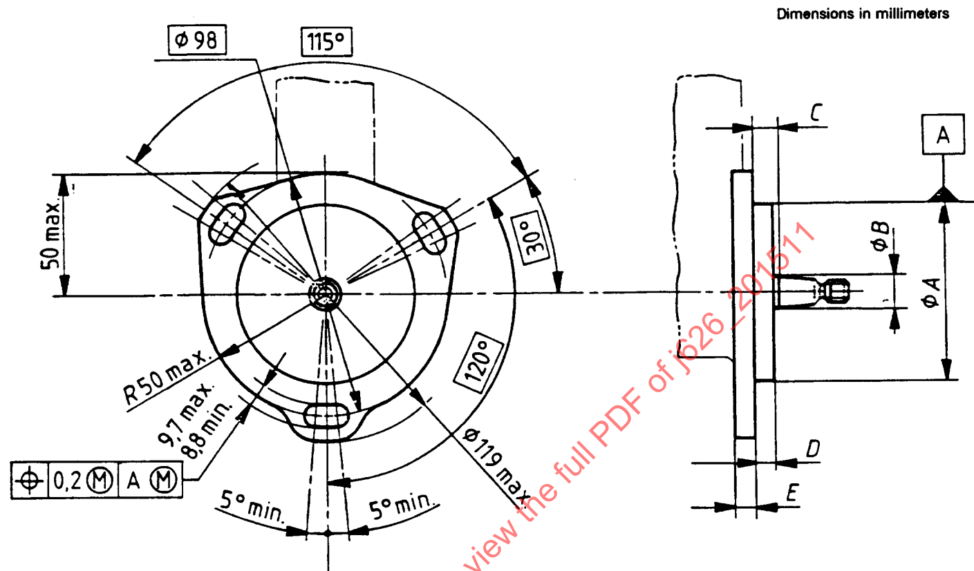
FIGURE 5—FUEL INJECTION PUMPS—TYPE 5 END-MOUNTING FLANGE
