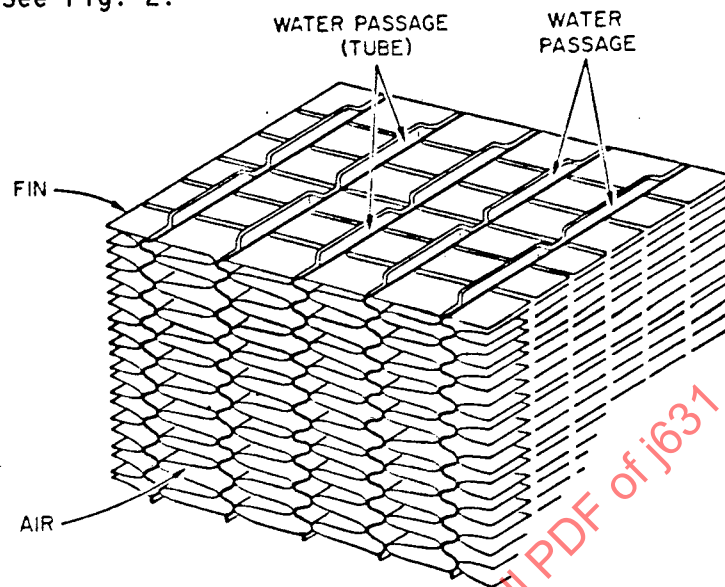
FIGURE 2 - Cellular Core
