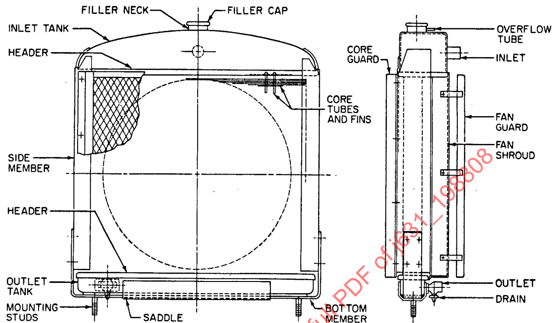
FIGURE 4 - Sheet Metal Radiator
