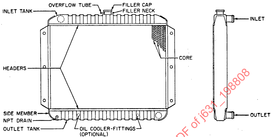
FIGURE 6 - Automotive Radiator (Down Flow)
