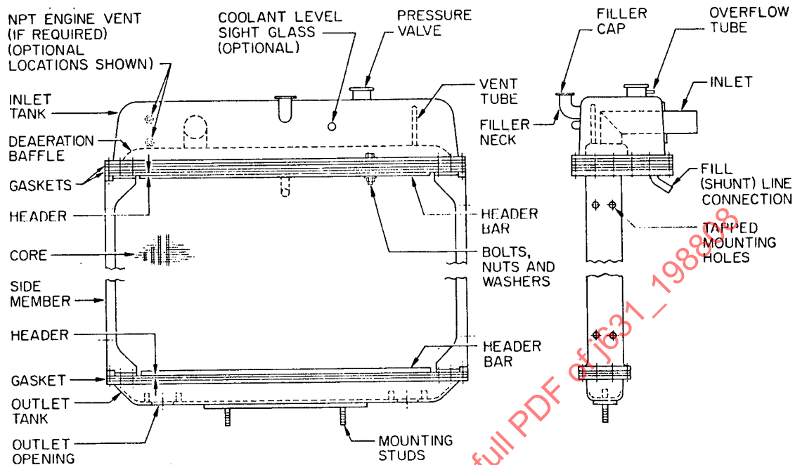
FIGURE 8 - Bolted Type Radiator, Drawn Tanks (Typical Deaeration System Shown)
