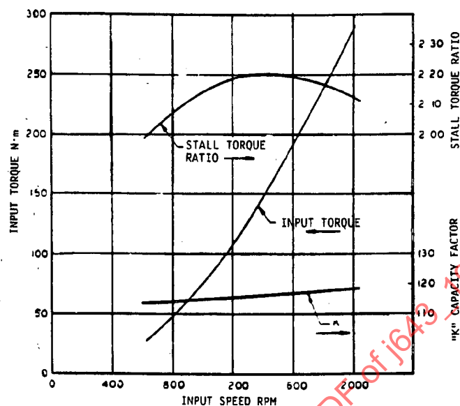
FIGURE 4 - Typical Input Speed Plot of Converter Stall Characteristics
