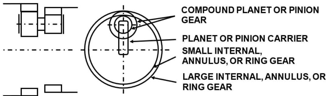
Figure 4 - Compound internal planetary arrangement, dual ring, stepped planet
