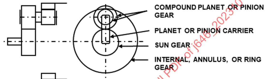
Figure 5 - Compound internal planetary arrangement, single sun, single ring, stepped planet
