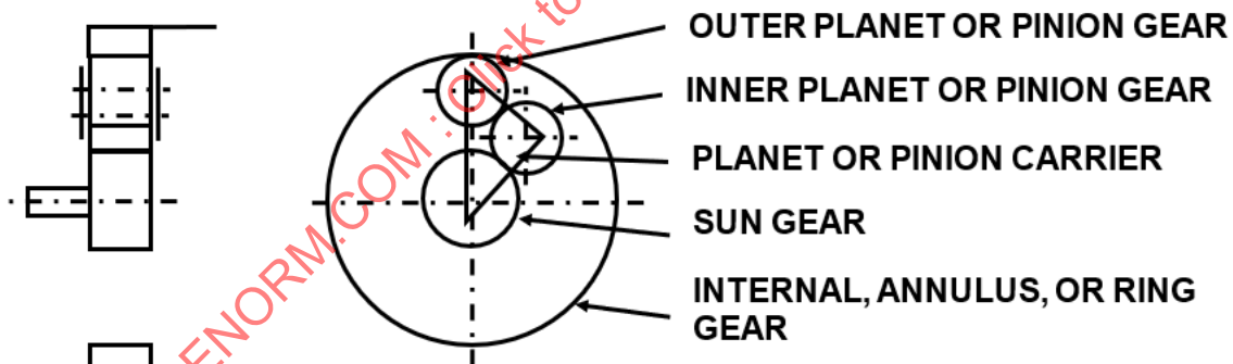
Figure 2 - Dual planetary arrangement
