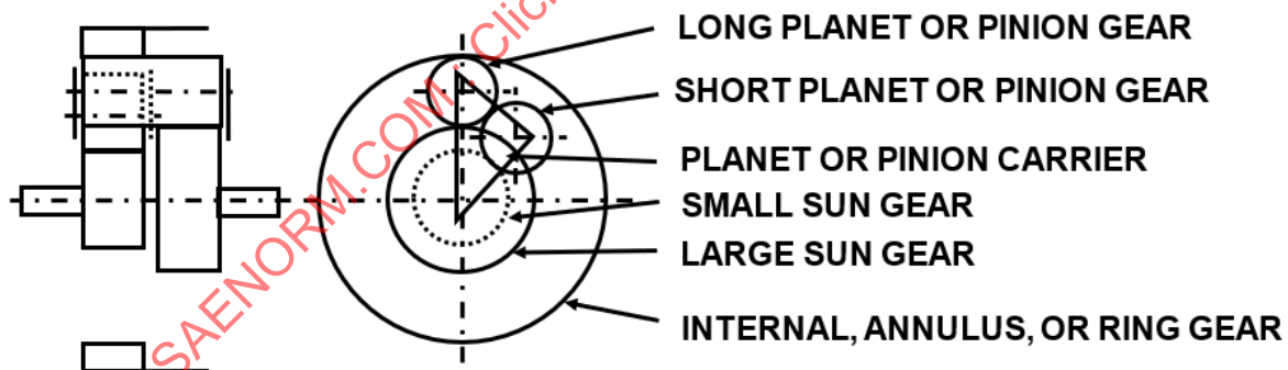
Figure 6 - Ravigneaux planetary arrangement
