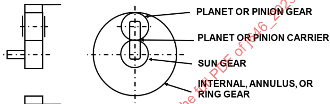
Figure 1 - Simple planetary arrangement
