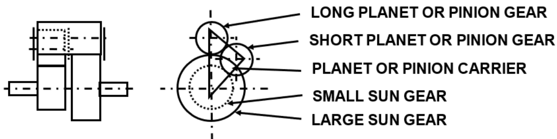
Figure 3 - Compound external planetary arrangement, dual sun, dual planet
