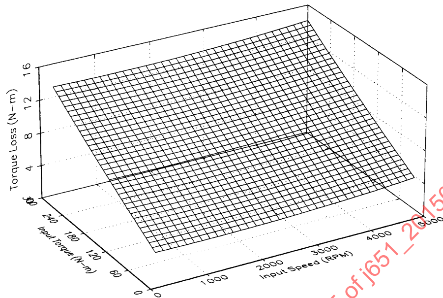
Transmission Torque Losses as a Function of Input Speed and Torque (Third Gear Locked Converter)
