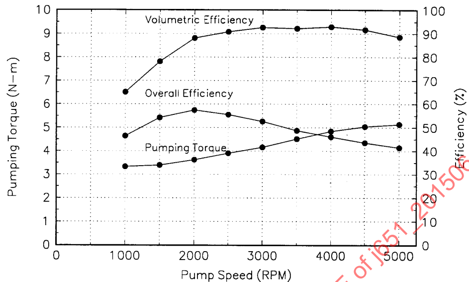
FIGURE 2 - PUMP PERFORMANCE
