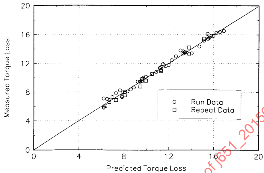
FIGURE 6 - PREDICTED VERSUS OBSERVED TORQUE
