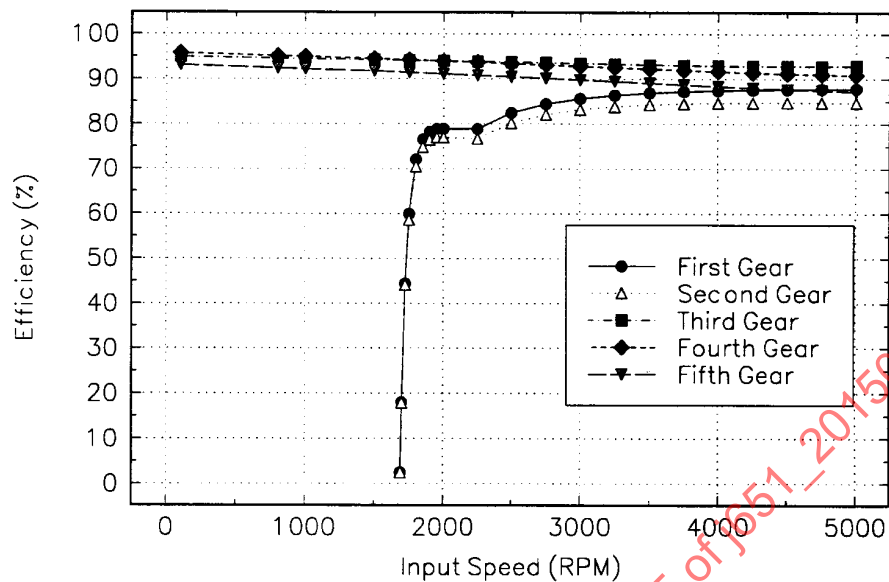
FIGURE 10 - TRANSMISSION EFFICIENCY DIFFERENT GEARS
