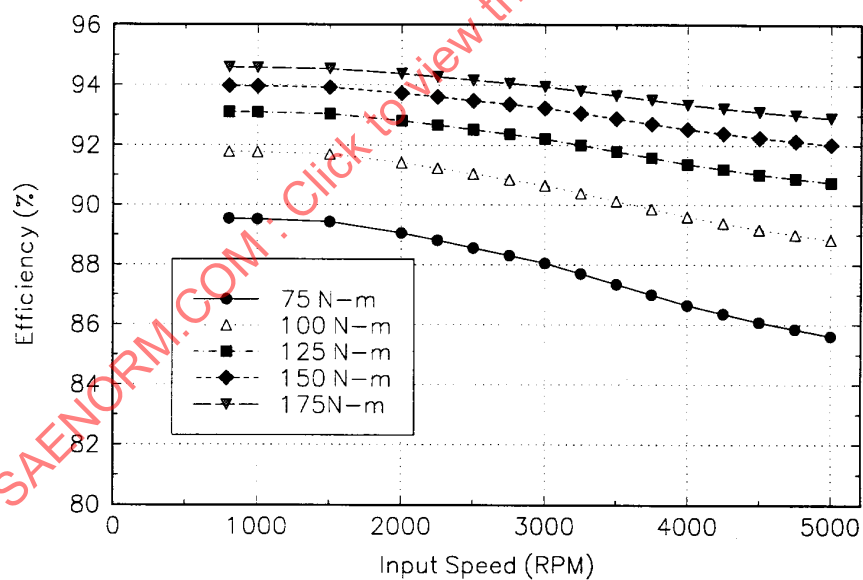
FIGURE 9 - TRANSMISSION EFFICIENCY FOURTH GEAR CONVERTER LOCKED
