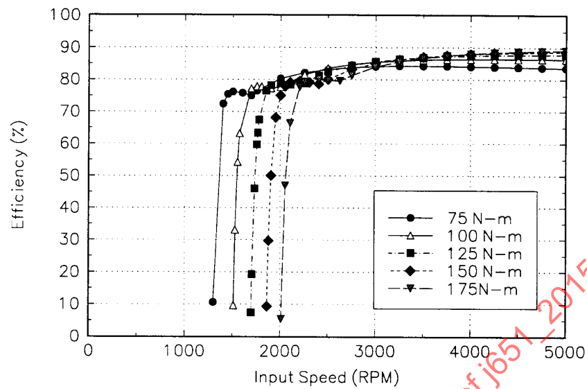
FIGURE 8 - TRANSMISSION EFFICIENCY FIRST GEAR UNLOCKED CONVERTER
