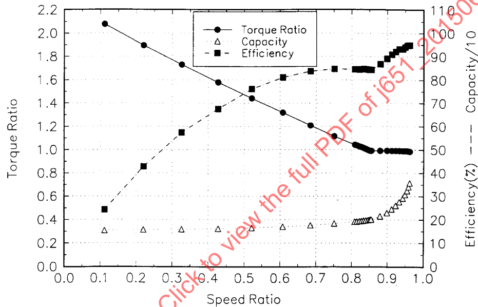
FIGURE 1 TORQUE CONVERTER PERFORMANCE
