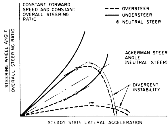
FIGURE 4—STEER PROPERTIES (SEE NOTE 17)
