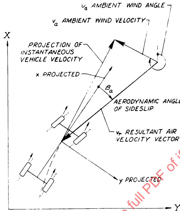
FIGURE 5—WIND VECTORS
