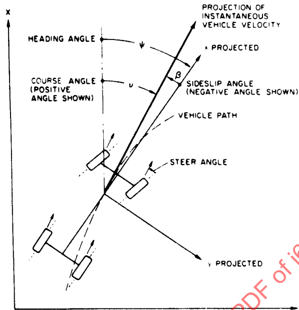
FIGURE 3—HEADING, SIDESLIP, AND COURSE ANGLES
