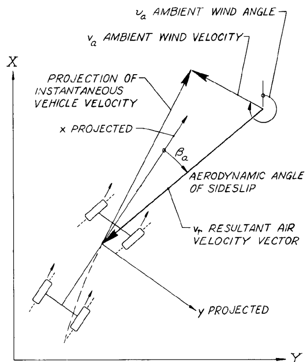
Fig. 5 - Wind vectors
