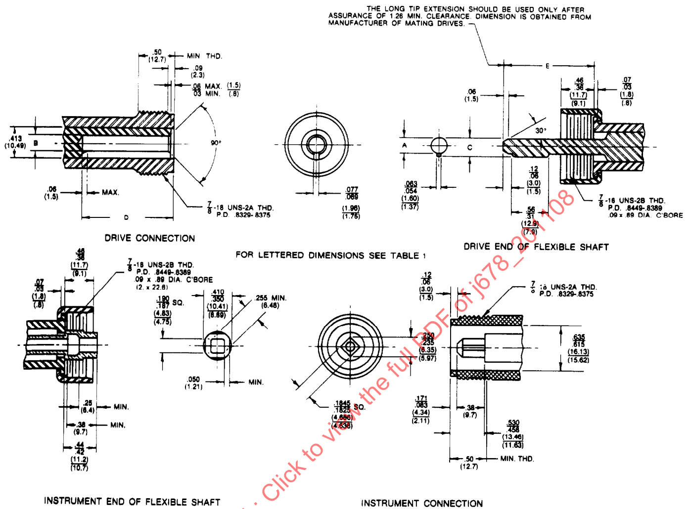
FIGURE 4—HEAVY-DUTY DRIVE (FOR USE WITH CENTRIFUGAL TYPE INSTRUMENTS)
