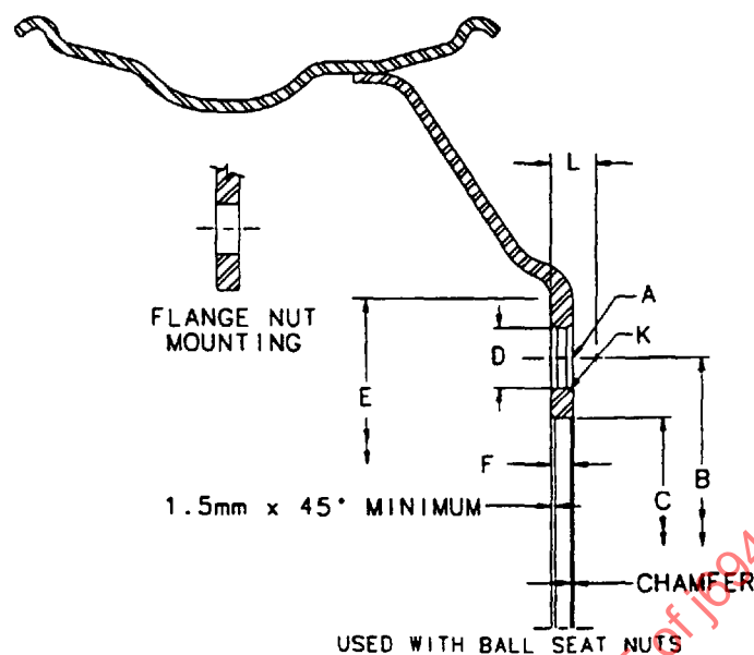
FIGURE 5—FERROUS DISC WHEEL
