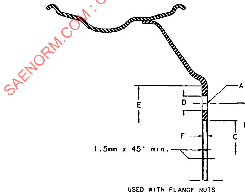
FIGURE 1—FERROUS DISC WHEEL
