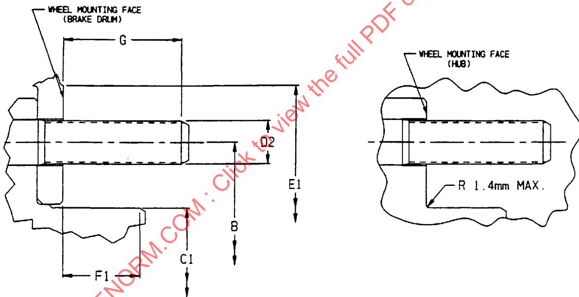
FIGURE 3—HUB OR DRUM INTERFACE DIMENSIONS
