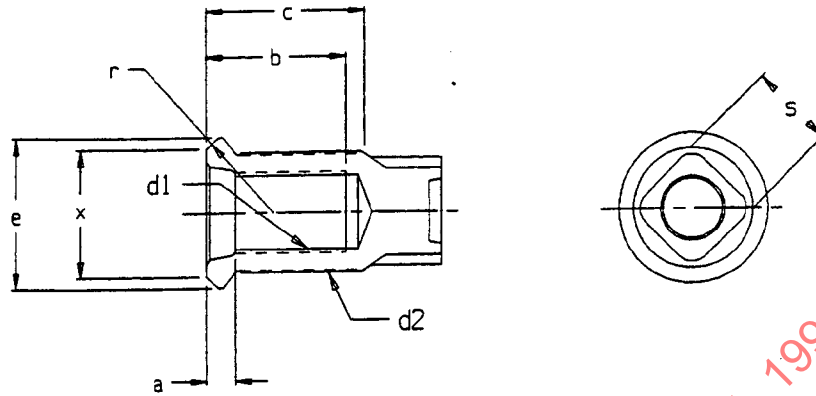
FIGURE 9—INNER DUAL BALL SEAT NUT FOR FERROUS WHEELS
