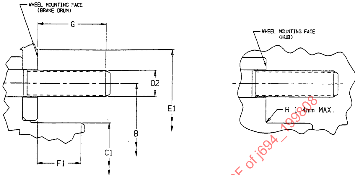
FIGURE 7—HUB OR DRUM INTERFACE DIMENSIONS
