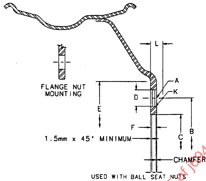
FIGURE 5—FERROUS DISC WHEEL
