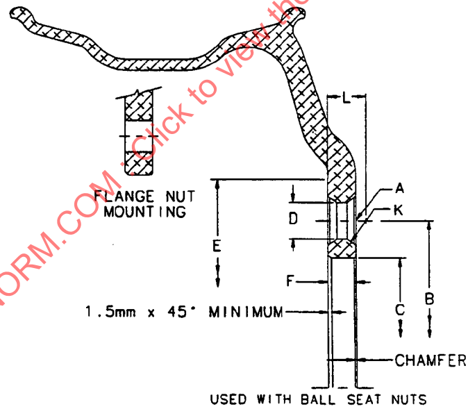
FIGURE 6—ALUMINUM DISC WHEEL
