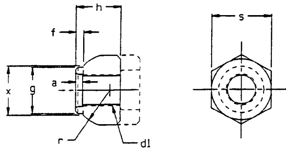
FIGURE 10—SINGLE OR OUTER DUAL BALL SEAT NUT FOR ALUMINUM WHEELS
