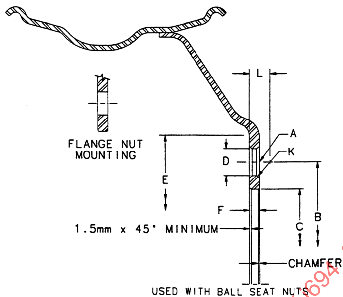
FIGURE 5 - FERROUS DISC WHEEL
