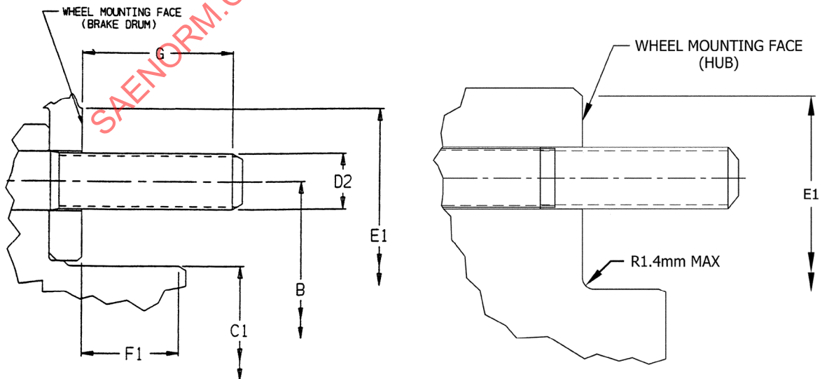
FIGURE 7 - HUB OR DRUM INTERFACE DIMENSIONS
