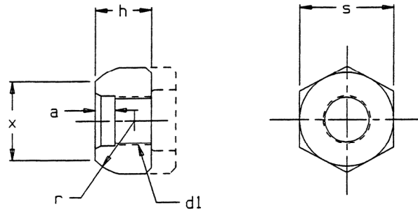
FIGURE 8 - SINGLE OR OUTER DUAL BALL SEAT NUT FOR FERROUS WHEELS
