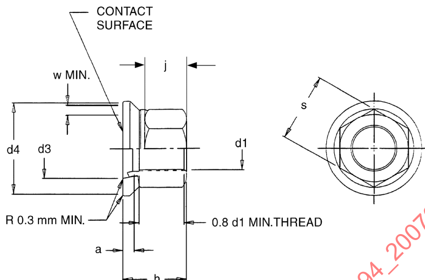
FIGURE 4 - TWO-PIECE FLANGE NUT
