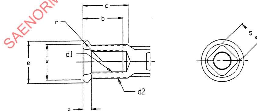
FIGURE 9 - INNER DUAL BALL SEAT NUT FOR FERROUS WHEELS
