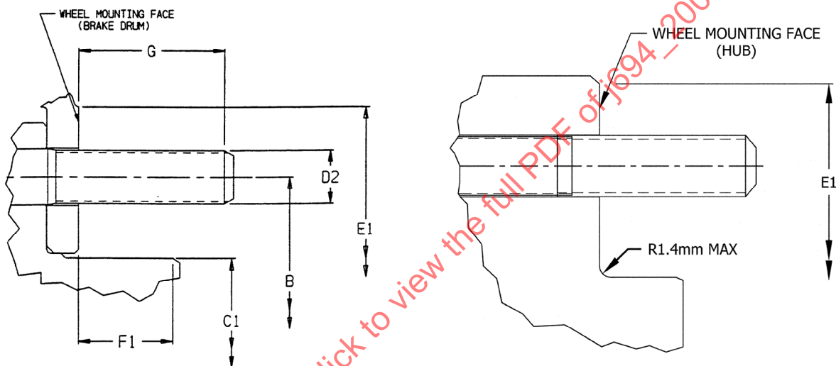
FIGURE 3 HUB OR DRUM INTERFACE DIMENSIONS
