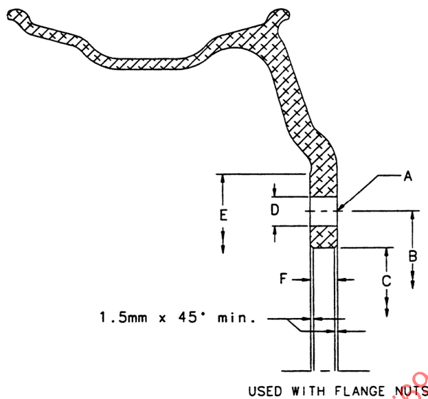
FIGURE 2 - ALUMINUM DISC WHEEL
