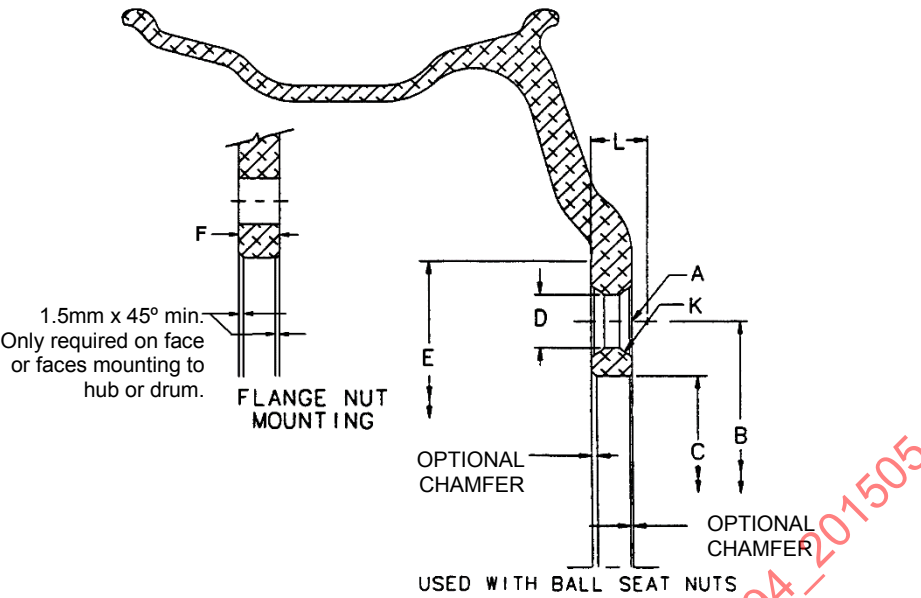
Figure 7 - Aluminum disc wheel
