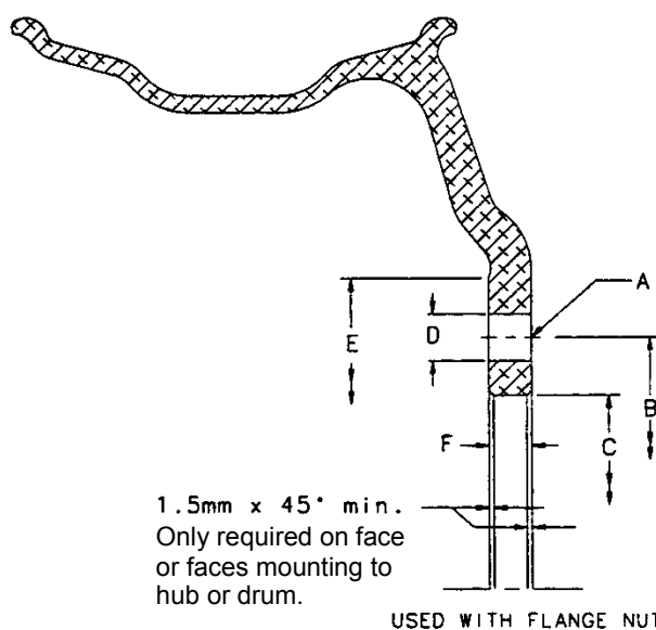
Figure 2 - Aluminum disc wheel
