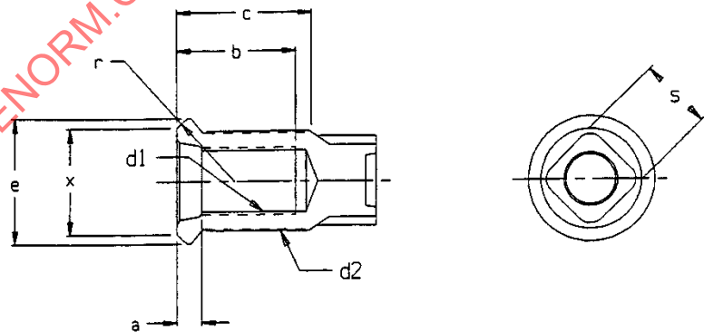
Figure 9 - Inner dual ball seat nut for ferrous wheels
