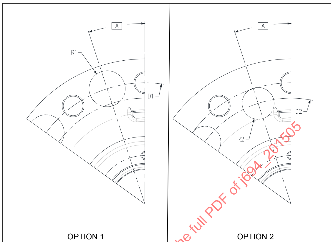
Figure 4 - Interface area of hub and wheel
