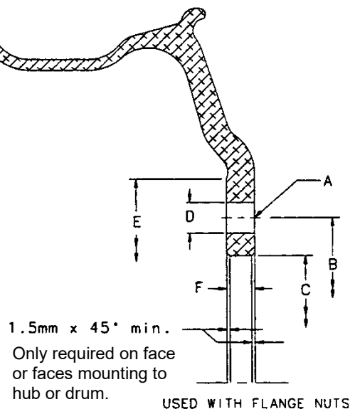
Figure 2 - Aluminum disc wheel
