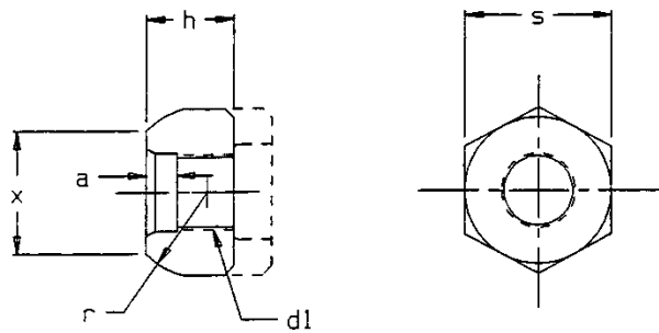
Figure 11 - Single or outer dual ball seat nut for ferrous wheels
