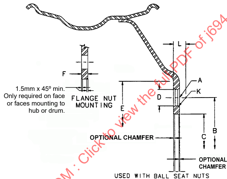
Figure 9 - Ferrous disc wheel
