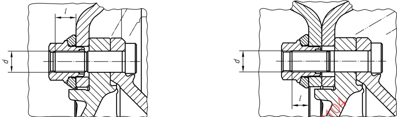
Figure 7 - Single and dual wheel mounting with short sleeve nut K
