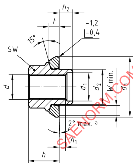
Short Sleeve (K)
