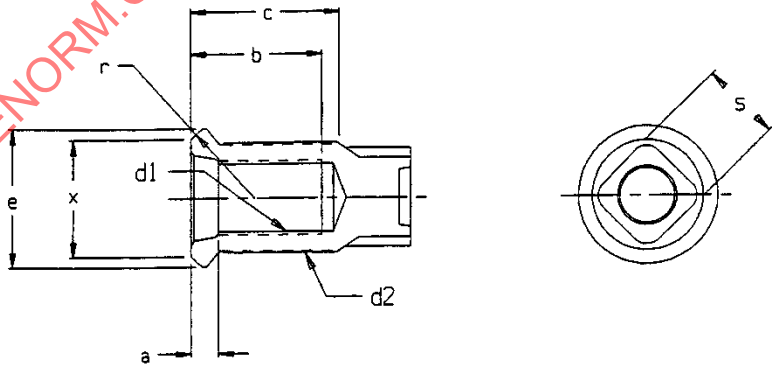
Figure 12 - Inner dual ball seat nut for ferrous wheels
