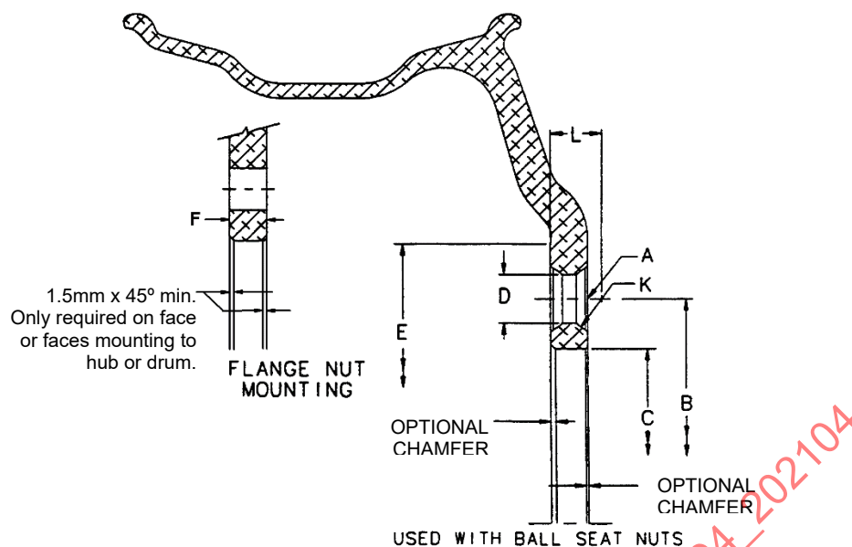
Figure 10 - Aluminum disc wheel
