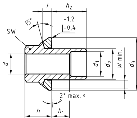
Long Sleeve (L)
