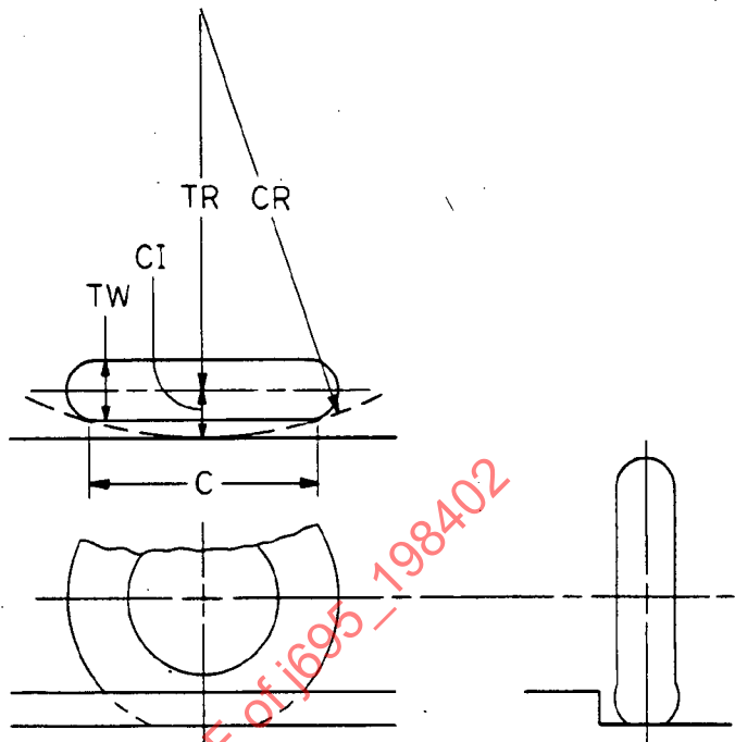
FIG. 4—CURB CLEARANCE DIAGRAM
