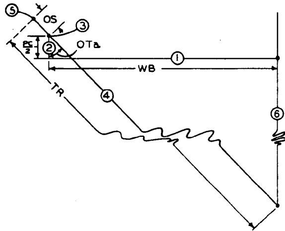
FIG. 5—GRAPHICAL PROCEDURE FOR DETERMINATION OF TURNING RADIUS
