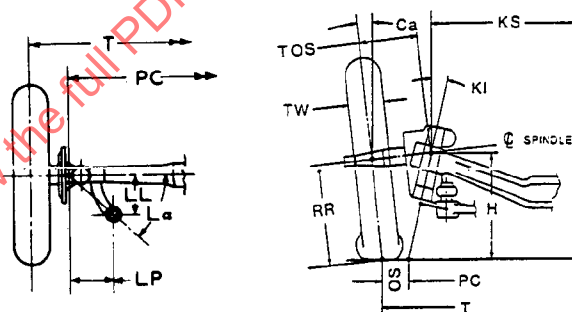
FIG. 2—DIAGRAM ILLUSTRATING FACTORS OF FRONT AXLE CONFIGURATION
