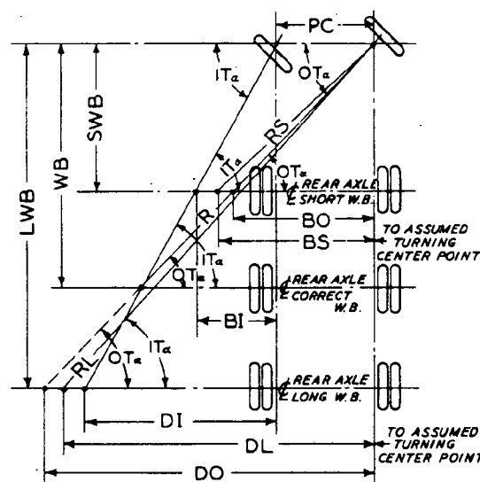
FIG. 3—DIAGRAM ILLUSTRATING EFFECT OF WHEELBASE ON TURNING RADIUS WITH A GIVEN FRONT AXLE CONFIGURATION
