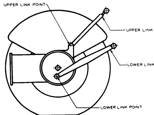
FIGURE 1 - Tractor Linkage
