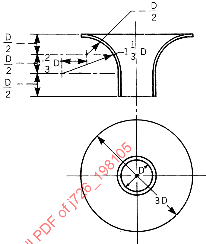
FIG. 2G—IDEAL FLOW ORIFICE
