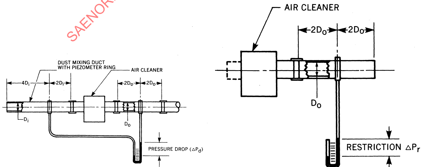
FIG. 3C—PRESSURE DROP TEST SET-UP
