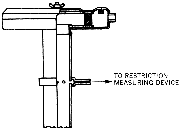
FIG. 2E—AIR CLEANER ASSEMBLY RESTRICTION TEST SET-UP
