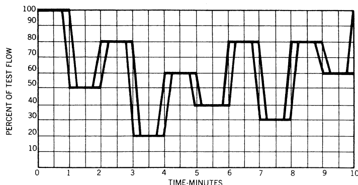
FIG. 2J—TYPICAL VARIABLE FLOW CYCLE AVERAGE FLOW 60%
