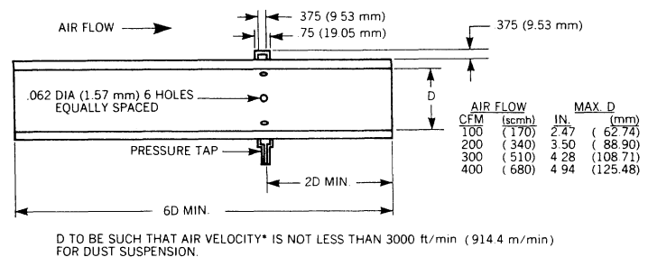
FIG. 2C—INLET TUBE
