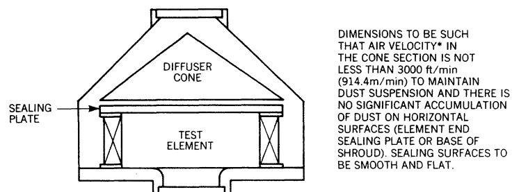
FIG. 2D—TEST SHROUD
