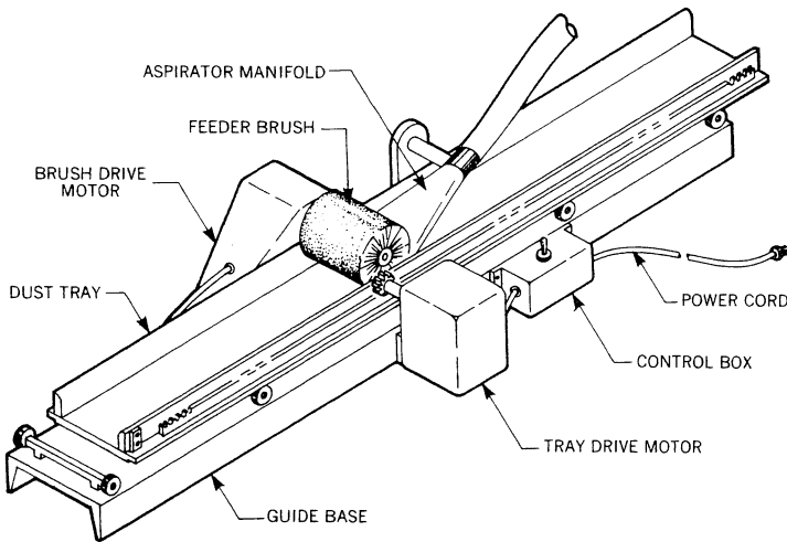
FIG. 3E—DUST FEEDER (DETAIL DRAWING AVAILABLE FROM SAE TEST CODE SUB-COMMITTEE)
