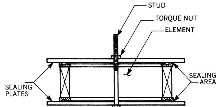
FIG. 2K—TEST ASSEMBLY
