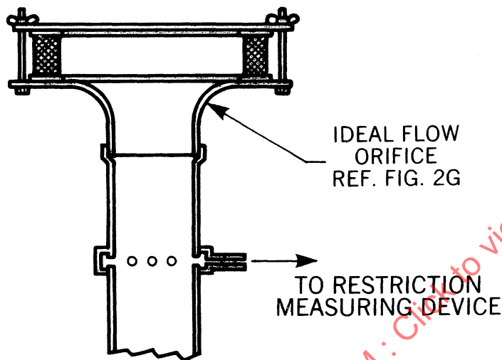
FIG. 2F—ELEMENT RESTRICTION TEST SET-UP
