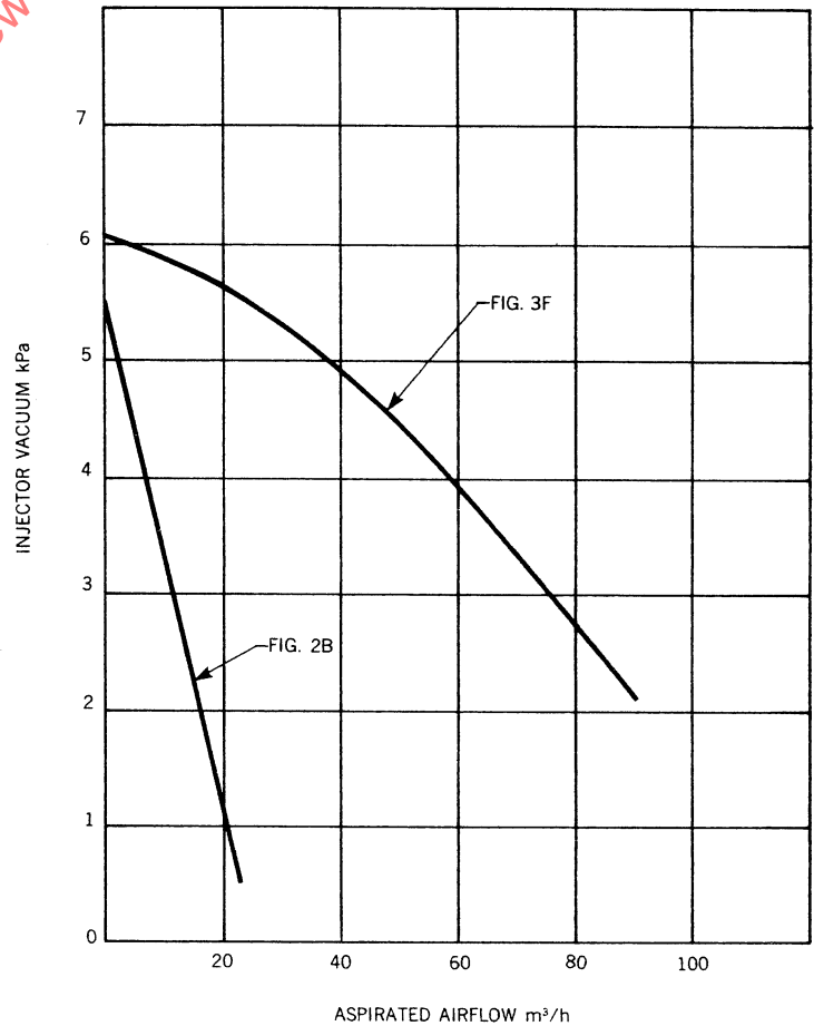
FIG. 3G—DUST INJECTOR PERFORMANCE
