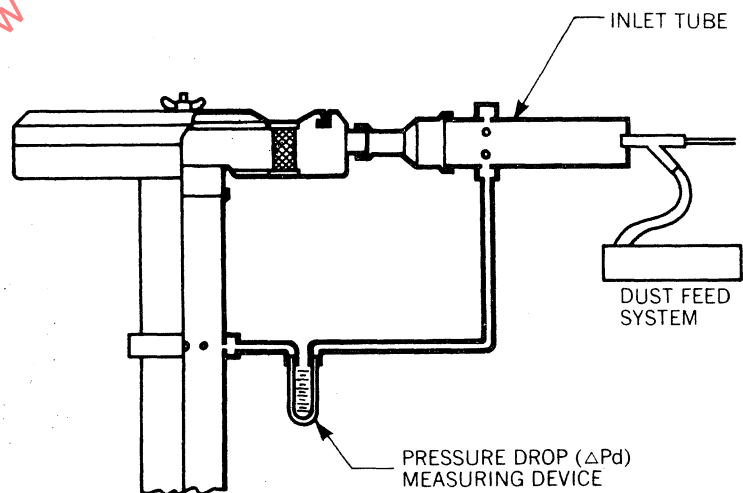
FIG. 2H—EFFICIENCY/CAPACITY AIR CLEANER ASSEMBLY TEST SET-UP
