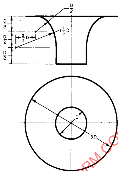
FIG. 2A—IDEAL FLOW ORIFICE
