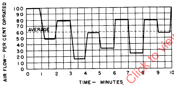
FIG. 5—VARIABLE FLOW CYCLE
