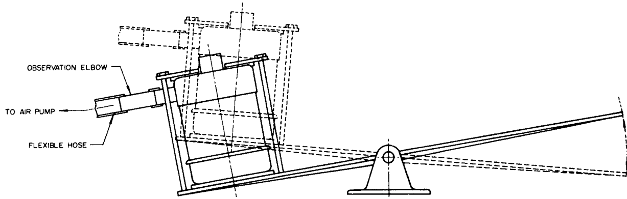
FIG. 7A—VERTICAL SHAKE AND ROLL
