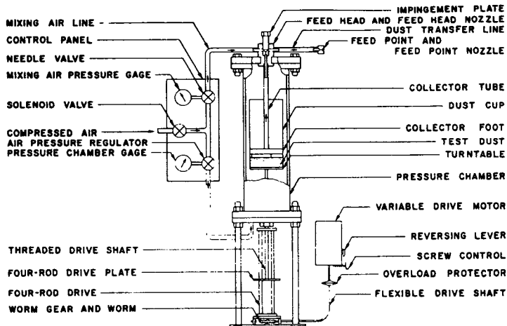
FIG. 4A—SONIC DUST FEEDER 4
