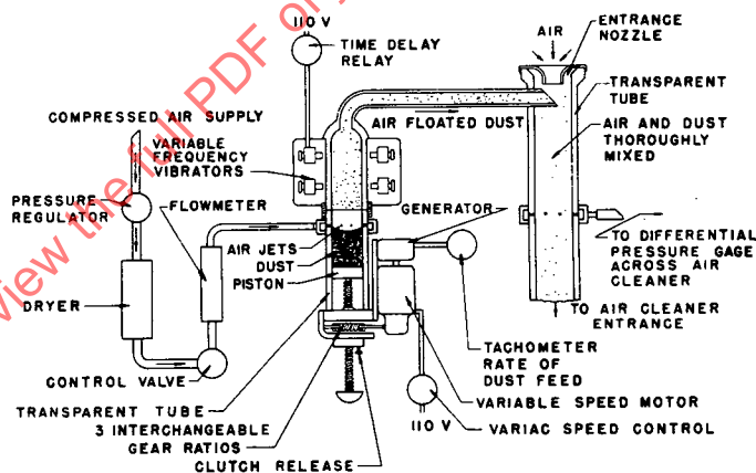
FIG. 3—MECHANICAL DUST FEEDER 3
