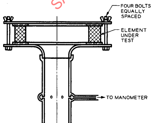
FIG. 2B—DRY CLEANER ELEMENT RESTRICTION TEST SETUP
