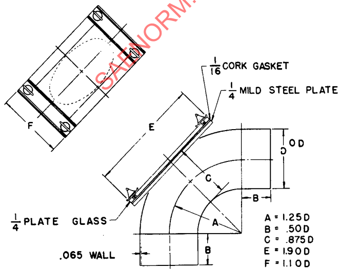
FIG. 6—OBSERVATION ELBOW
