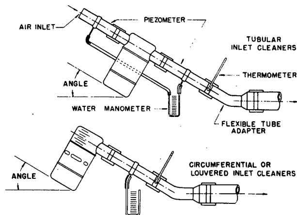
FIG. 9—TEST SETUP
