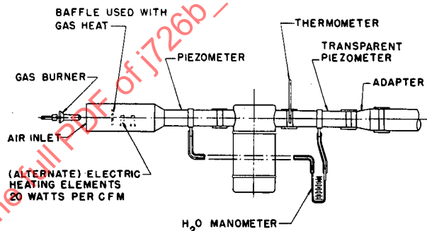
FIG. 10—OIL LOSS TEST SETUP
