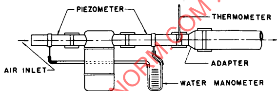
FIG. 8C—TUBULAR INLET CLEANERS
