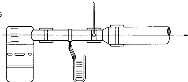
FIG. 8A—CIRCUMFERENTIAL OR LOUVERED INLET CLEANERS
