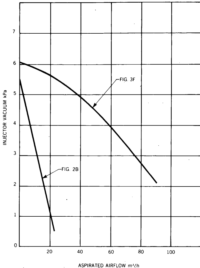
FIG. 3G—DUST INJECTOR PERFORMANCE
