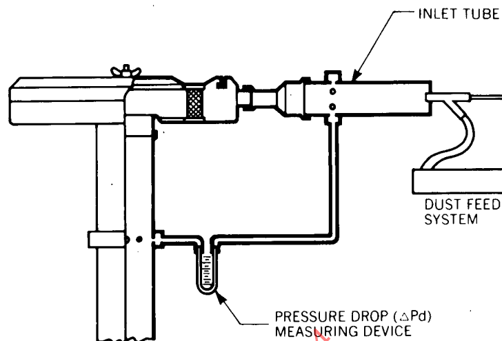
FIG. 2H—EFFICIENCY/CAPACITY AIR CLEANER ASSEMBLY TEST SET-UP
