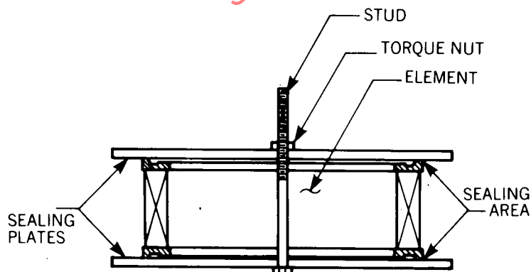
FIG. 2K—TEST ASSEMBLY
