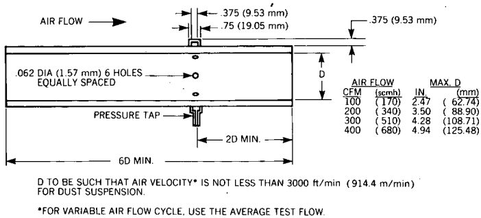
FIG. 2C-INLET TUBE
