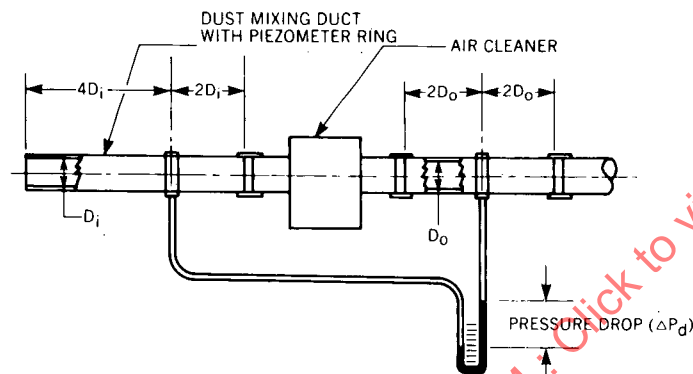
FIG. 3C—PRESSURE DROP TEST SET-UP
