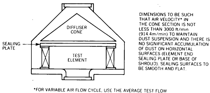
FIG. 2D-TEST SHROUD
