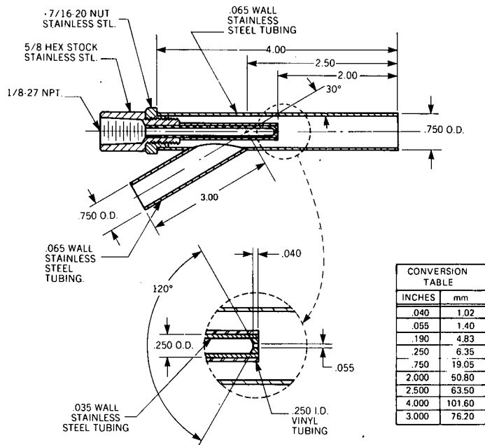
FIG. 2B—DUST INJECTOR
