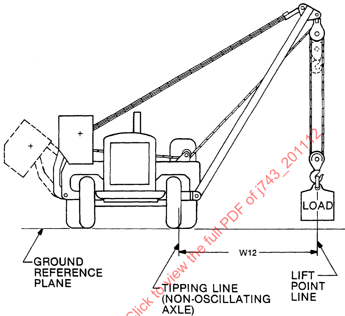
FIGURE 2—WHEEL MACHINE STEERED STRAIGHT
