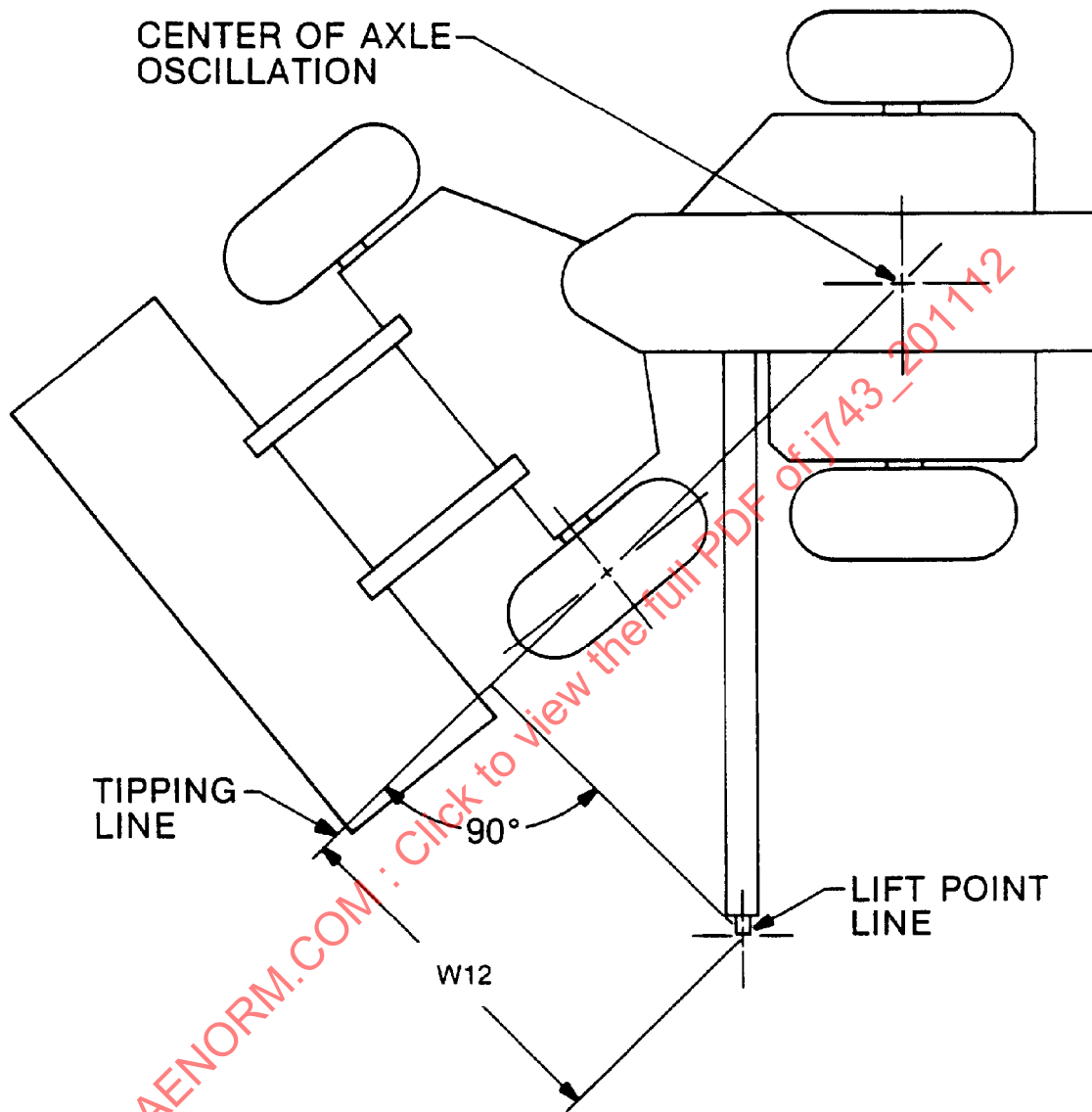
FIGURE 7—ARTICULATED WHEEL TRACTOR STEERED LEFT OSCILLATING AXLE
