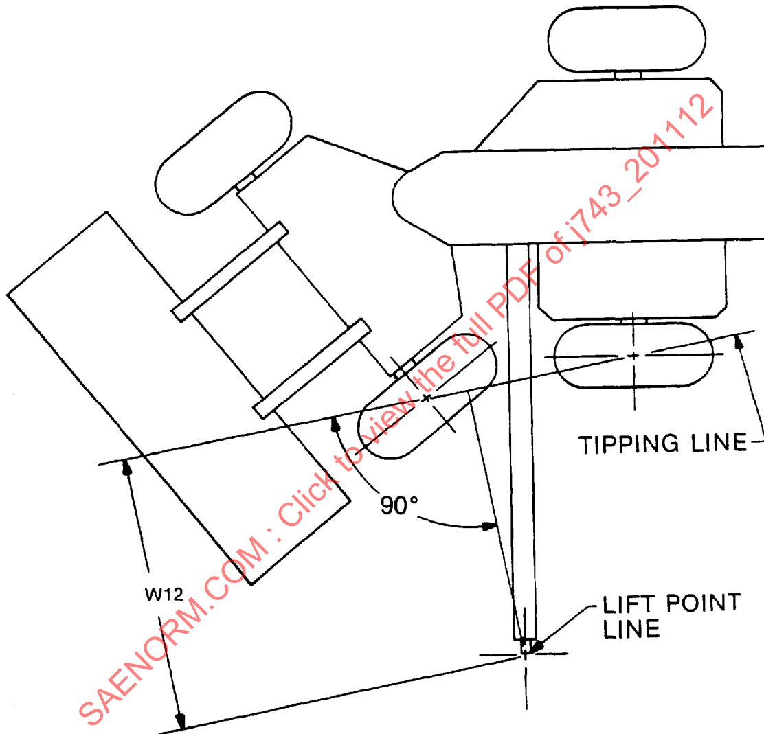
FIGURE 5—ARTICULATED WHEEL TRACTOR STEERED LEFT NON-OSCILLATING AXLE
