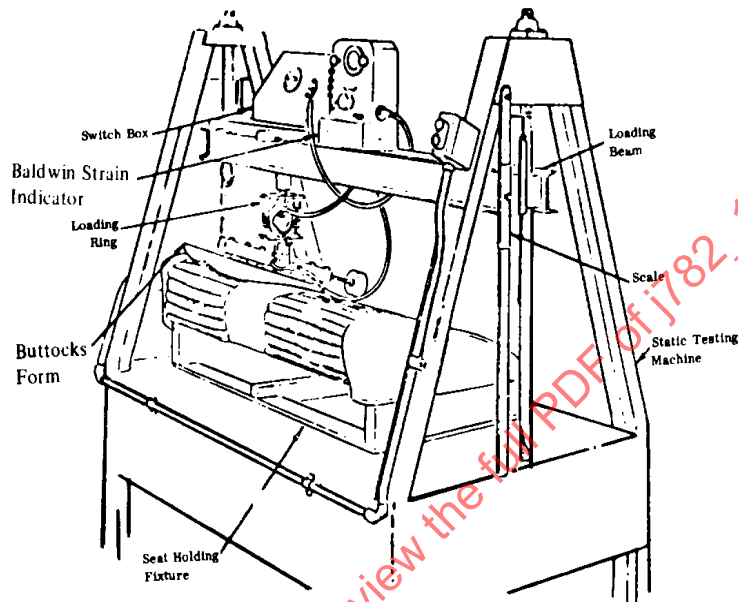
FIGURE 38—LOAD DISTRIBUTION TEST SETUP
