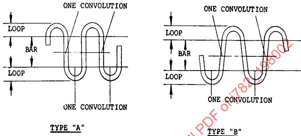
FIGURE 22—ZIGZAG CONFIGURATION
