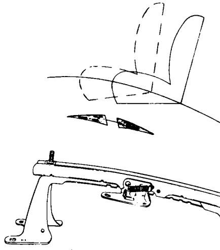
FIGURE 5—TWO-WAY CURVED ADJUSTER
