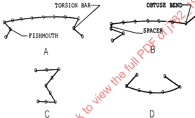
FIGURE 24—TYPES OF ZIGZAG OR FORMED WIRE PROFILES
