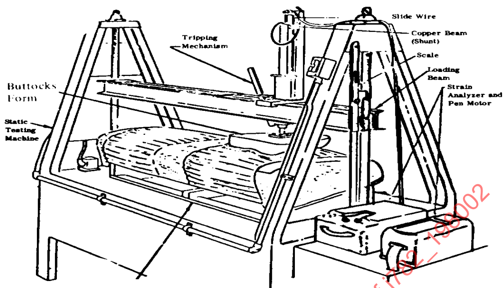
FIGURE 40—SEAT DROP TEST SETUP
