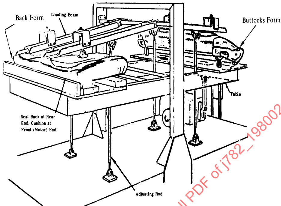
FIGURE 41—SEAT FATIGUE TEST SETUP (CONSTANT DEFLECTION OR CONSTANT WORK)
