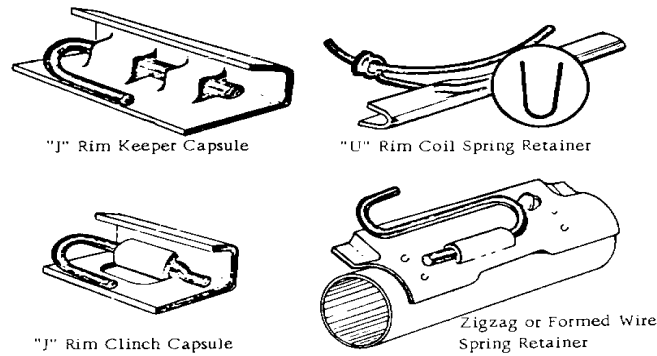
FIGURE 34—SPRING RETAINERS
