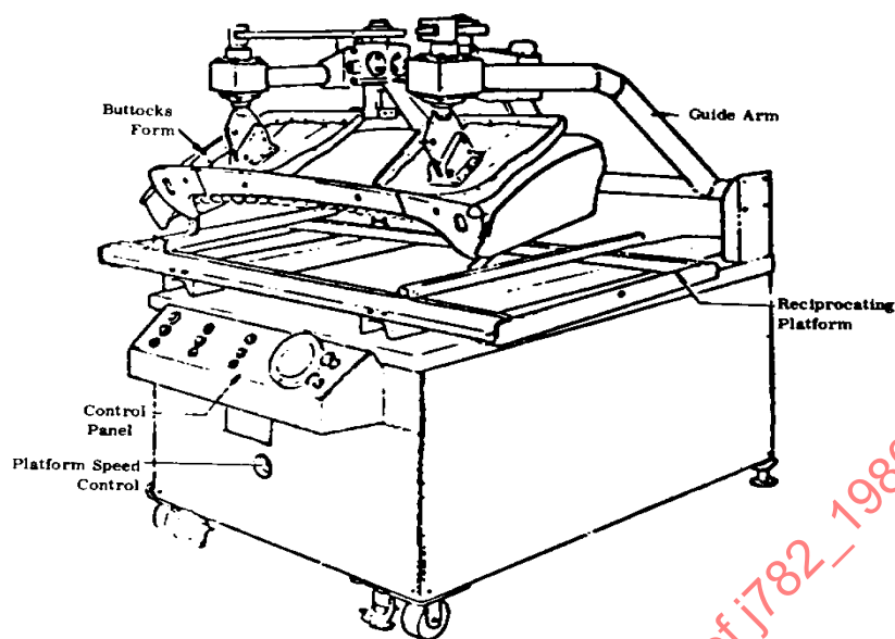
FIGURE 42—SEAT FATIGUE TEST SETUP (CONSTANT WORK)
