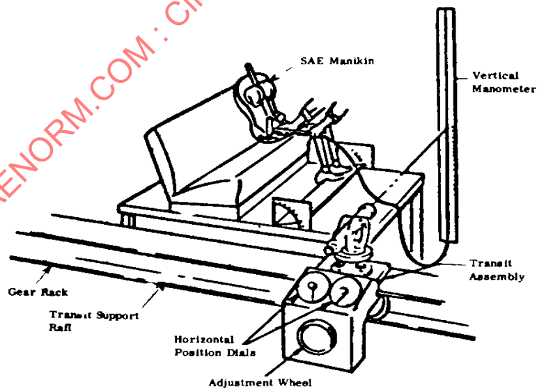
FIGURE 37—PACKAGE CHECK SETUP
