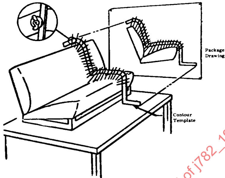
FIGURE 36—FREE CONTOUR SETUP
