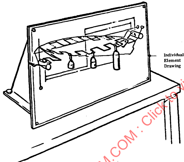
Fig. 5-4 - Single element load deflection setup
