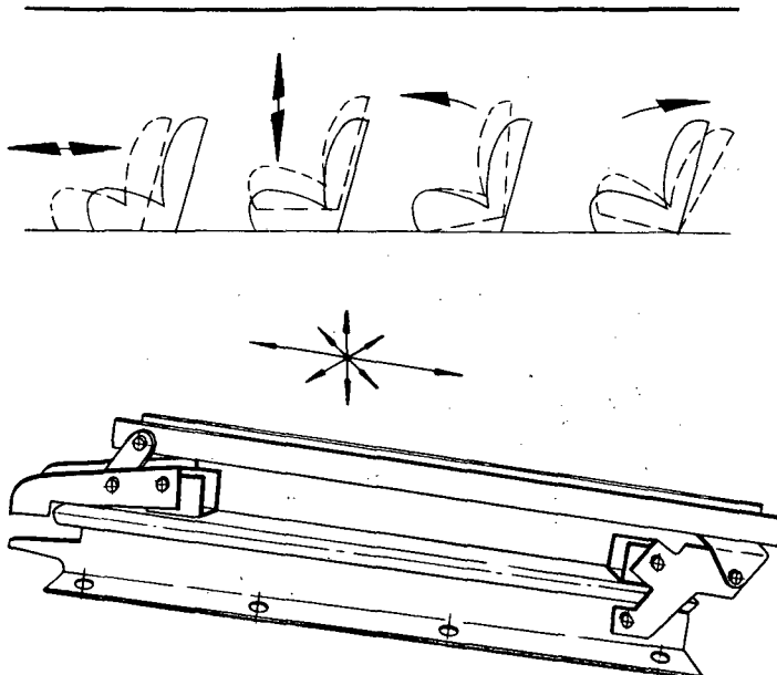
Fig. 2-5 - Six-way adjuster
