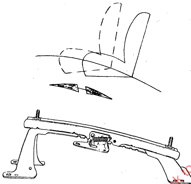
Fig. 2-3 - Two-way curved adjuster
