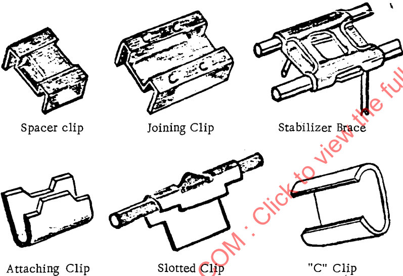
Fig. 4-12 - Clips
