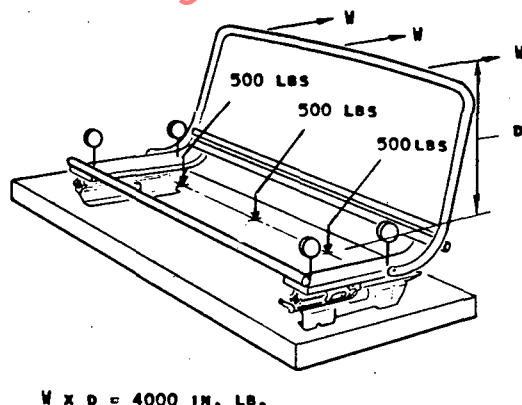
Fig. 2-7 - Static vertical load test of seat adjuster
