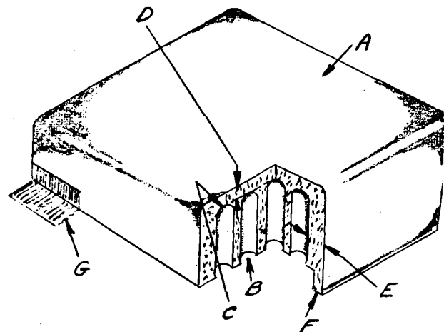
Fig. 7-7 - Cored stock
