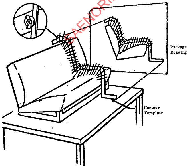
Fig. 5-1 - Free contour setup
