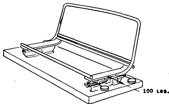
Fig. 2-8 - Static lateral load test of seat adjuster
