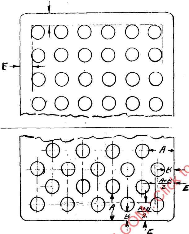
Fig. 7-8 - Staggered cores
