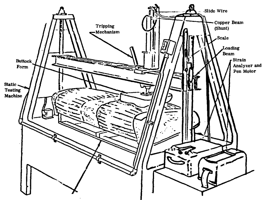
Fig. 5-4 - Single element load deflection setup
