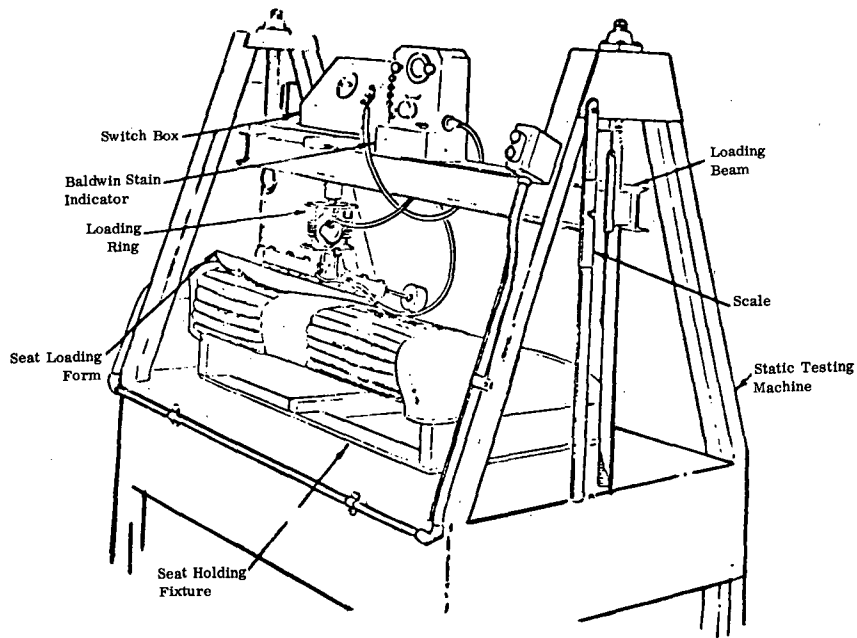
Fig. 5-3 - Load distribution test setup
