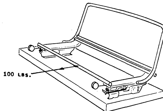
Fig. 2-9 - Static fore and aft chucking test of seat adjuster
