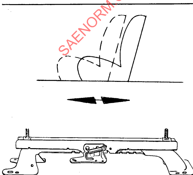
Fig. 2-1 - Two-way straight adjuster
