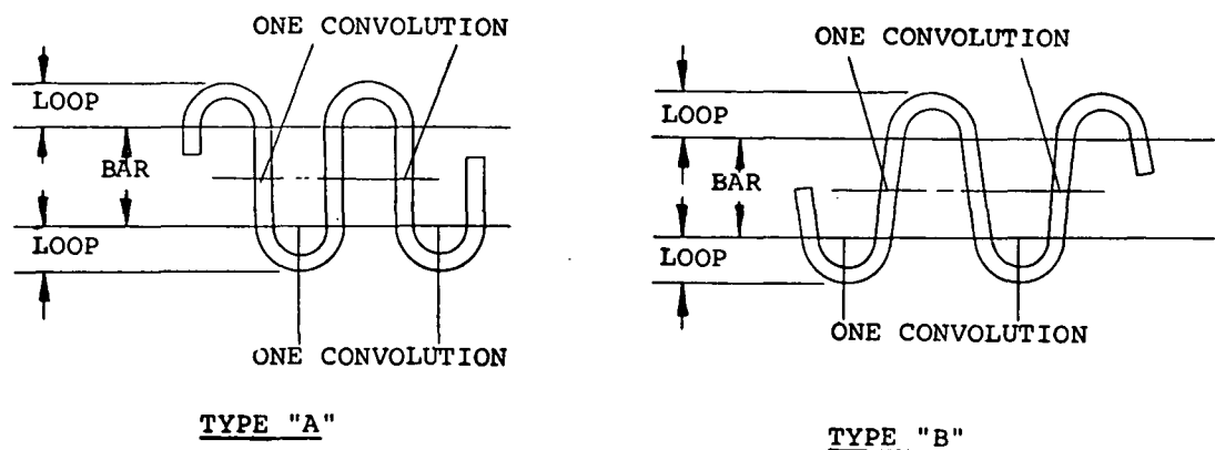
Fig. 4-1 - Zigzag configuration
