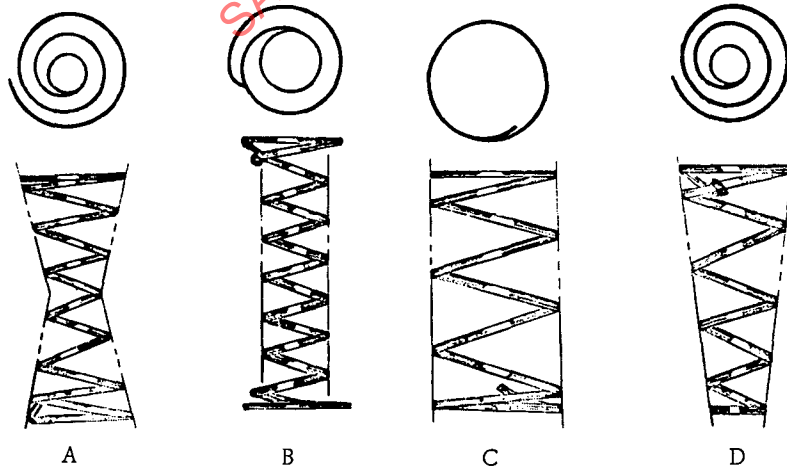
Fig. 4-4 - Configurations of spiral wire formations
