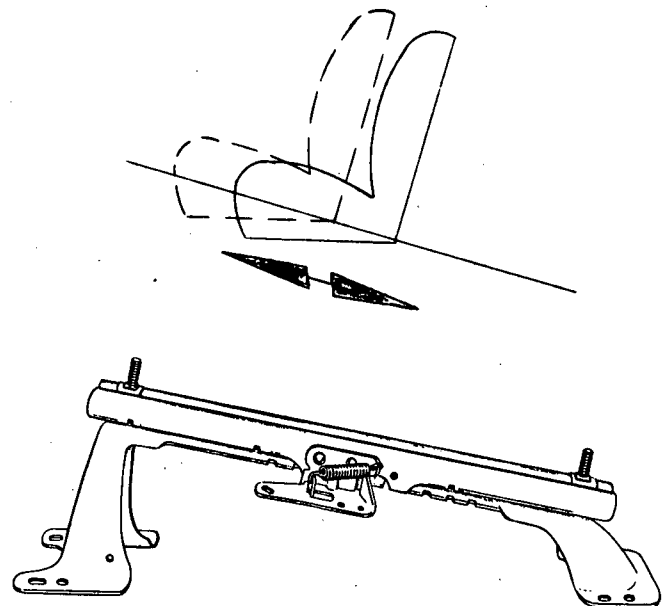
Fig. 2-2 - Two-way inclined straight adjuster
