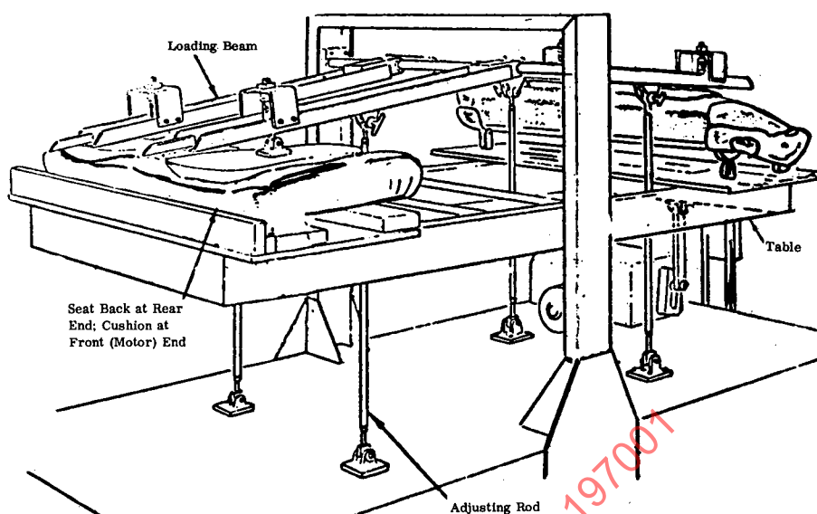
Fig. 5-6 - Seat fatigue test setup (constant deflection or constant work)
