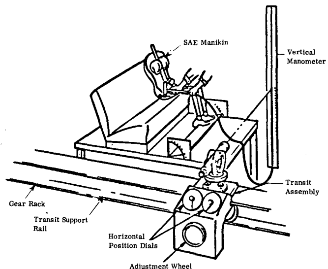
Fig. 5-2 - Package check setup
