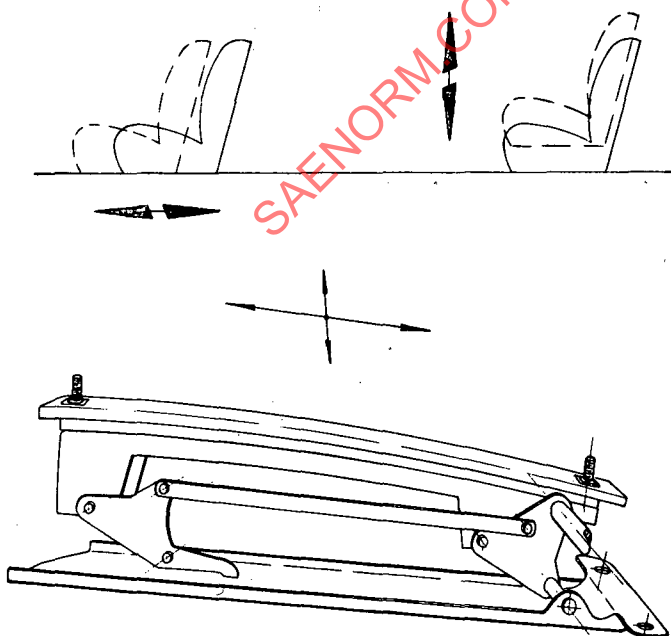
Fig. 2-4 - Four-way elevating adjuster
