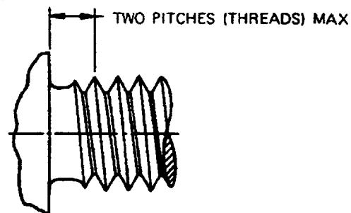
FIGURE 3—TYPE CSD THREAD FORM
