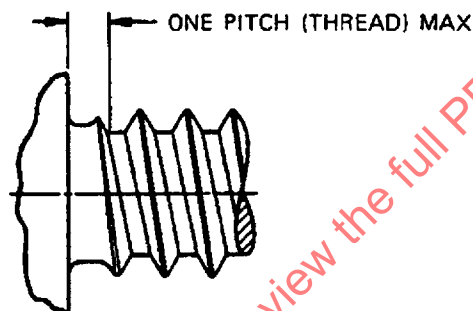
FIGURE 2—TYPE BSD THREAD FORM
