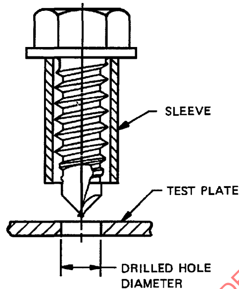
FIGURE 7—DRILL HOLE SIZE TEST
