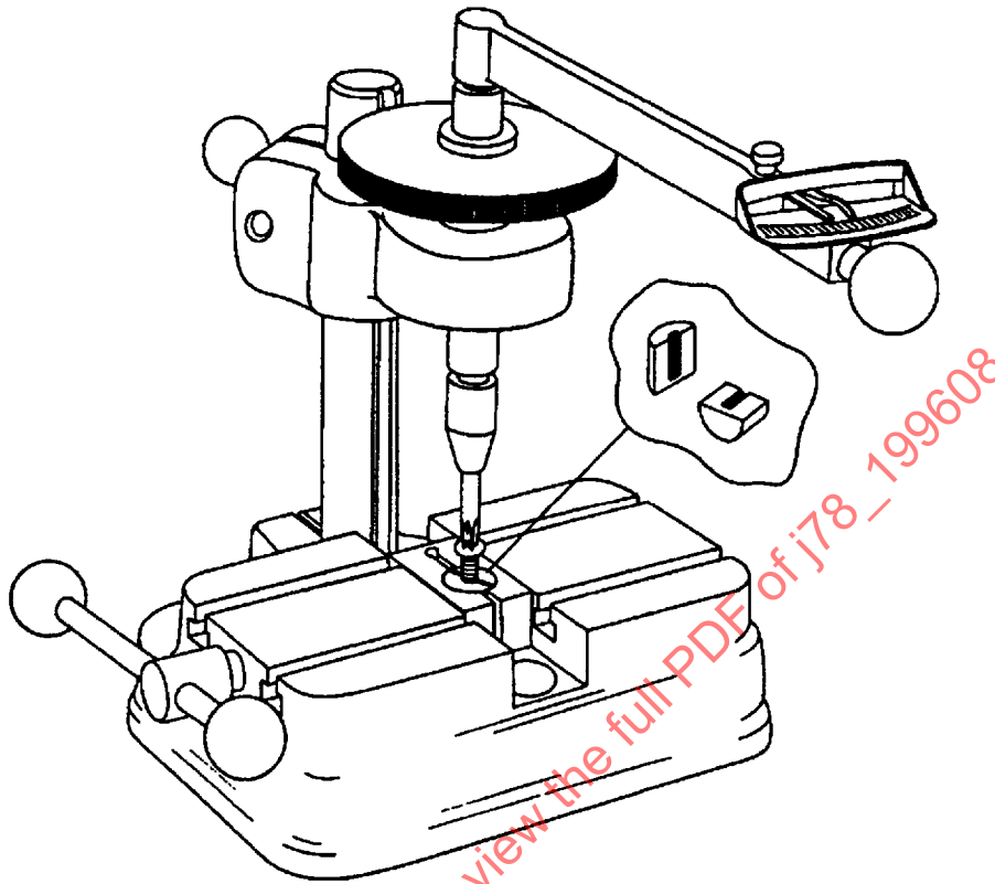
FIGURE 5—TYPICAL TORSIONAL STRENGTH TEST FIXTURE
