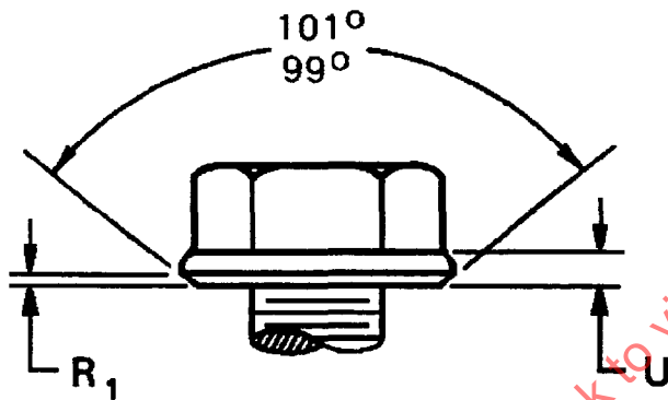
FIGURE 1A—HEX WASHER HEAD
