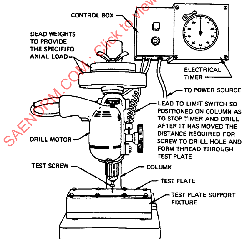
FIGURE 6—TYPICAL DRILL-DRIVE TEST FIXTURE
