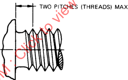
FIGURE 3—TYPE CSD THREAD FORM
