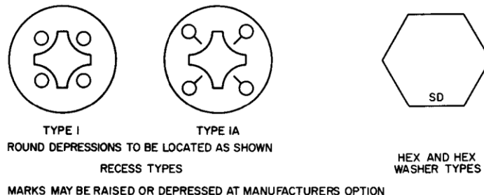
FIGURE 9—HEAD MARKING
