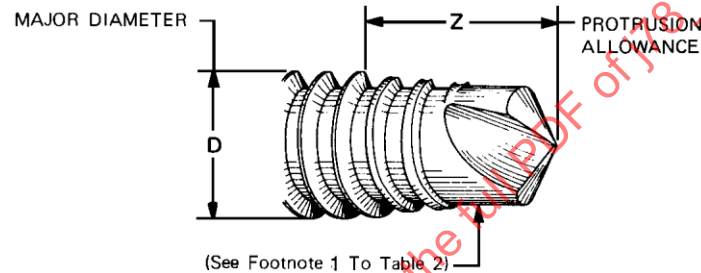
FIGURE 4—TYPICAL SELF-DRILLING TAPPING SCREW POINT
