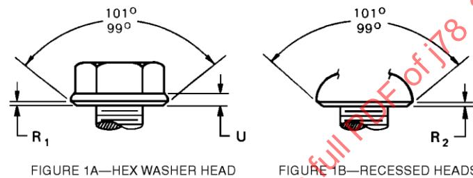
FIGURE 1—HEAD CHAMFERS ON MILLED POINT SCREWS
