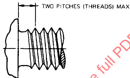
Figure 4 - Type CSD thread form
