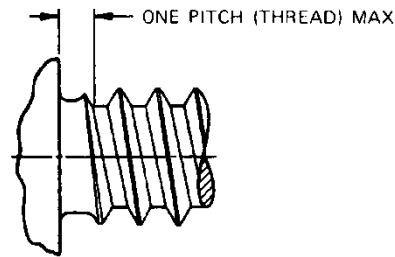
Figure 3 - Type BSD thread form
