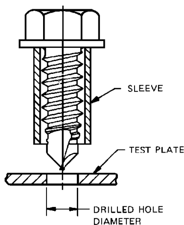
Figure 8 - Drill hole size test
