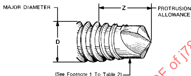
Figure 5 - Typical self-drilling tapping screw point
