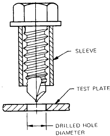
FIG. 7—DRILL HOLE SIZE TEST
