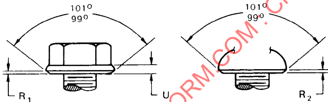
FIG. 1A—HEX WASHER HEAD FIG. 1B—RECESSED HEADS
