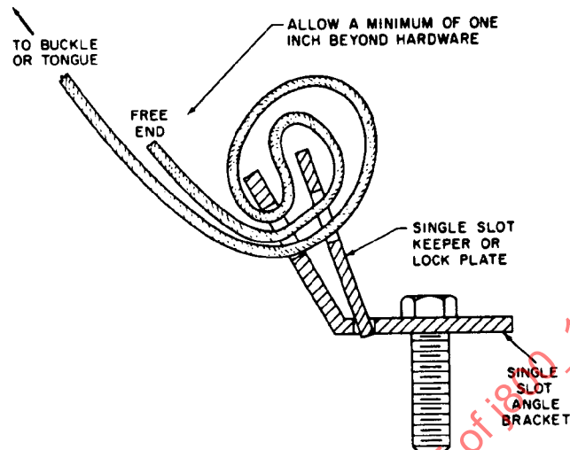
FIG. 1--SAME THREADING MAY BE USED FOR TWO-PIECE ANCHOR HOOKS IF EACH PIECE HAS SINGLE SLOT ONLY. AFTER WEBBING HAS BEEN THREADED AND HOOKS HAVE BEEN ASSEMBLED TO EYE BOLT, THE TWO HOOKS MUST BE FASTENED TOGETHER WITH COTTER KEY OR OTHER DEVICE
