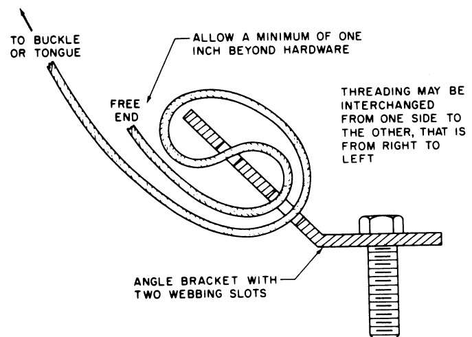
FIG. 2—SAME THREADING IS USED FOR TWO-SLOT SISTER HOOKS OR TWIN HOOKS, TWO PARTS BEING HELD TOGETHER BY WEBBING AS THOUGH THEY ARE SINGLE UNIT
