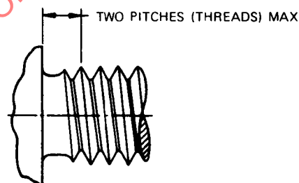
FIGURE 1—THREAD MAJOR DIAMETER LIMIT
