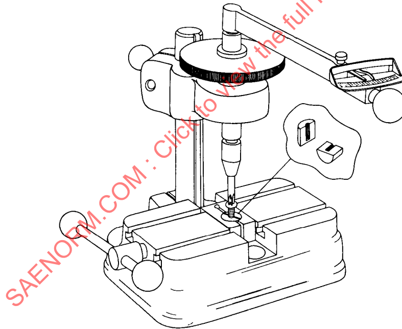
FIGURE 2—TYPICAL TORSIONAL STRENGTH TEST FIXTURE
