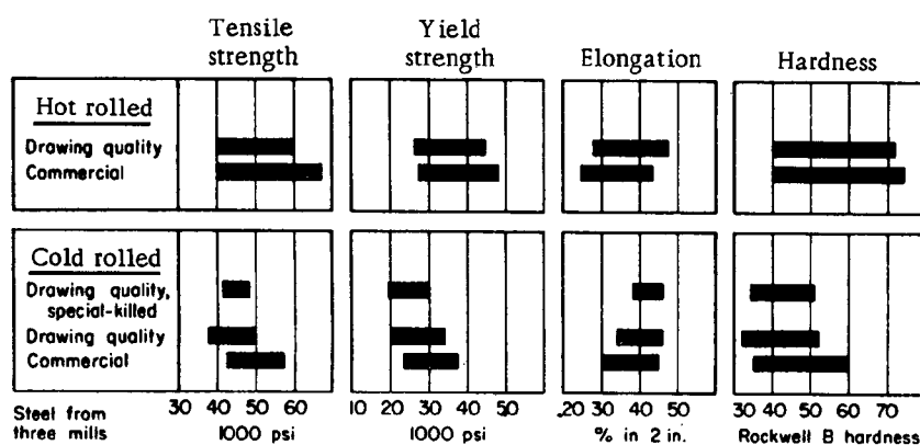
Fig. 1 - Typical range of mechanical properties of 1008 steel furnished by three mills. Hot rolled sheet thicknesses from 0.0958 to 0.1345 in. (16 to 10-gage inclusive); cold rolled from 0.029 to 0.059 in. (22 to 16-gage inclusive). All cold rolled grades include a temper pass. All grades rolled from rimmed steel except the one labelled special killed.
