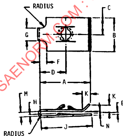
FIGURE 11A STYLE I—STANDARD THROAT AND STYLE III—LONG THROAT
