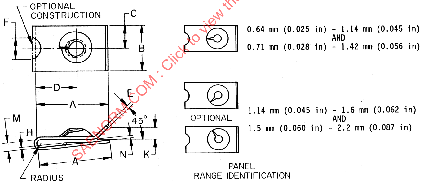
FIGURE 9—U SHAPE STYLE—STANDARD, STYLE II—SHORT, AND STYLE III—LONG THROAT
