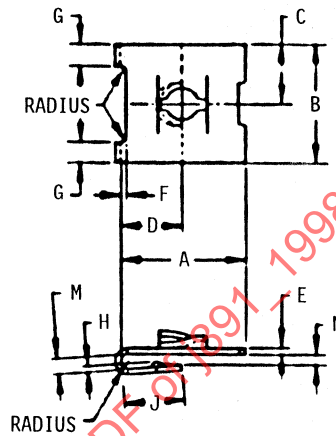
FIGURE 10B STYLE II—SHORT THROAT
