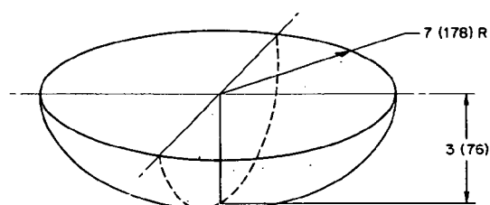
SEGMENT OF SPHERE OF RADIUS = 9.665 (245.5) NOTE: DIMENSIONS ARE IN (mm)
