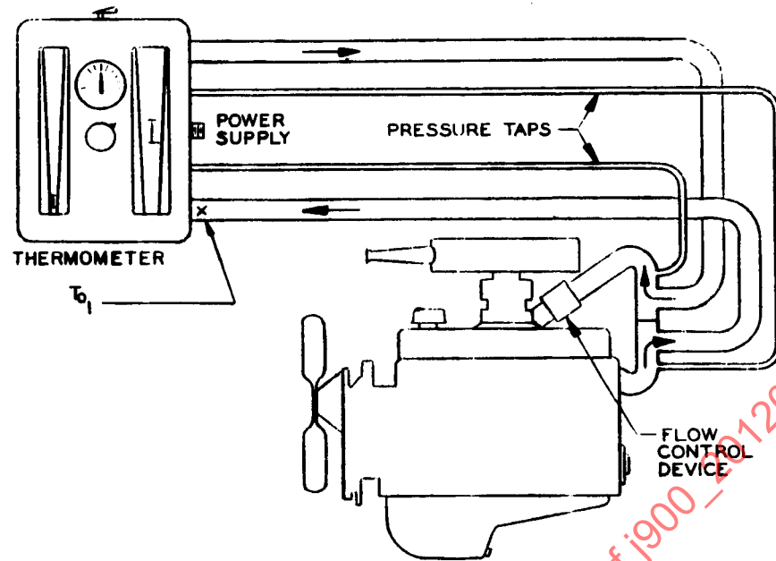
FIGURE 4—TYPICAL INSTALLATION FOR MEASURING SYSTEM OUTFLOW
