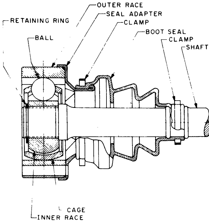
FIG. 18—CROSS GROOVE UNIVERSAL JOINT
