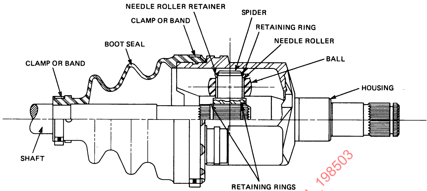
FIG. 12—TRIPOT OR TRIPOD UNIVERSAL JOINT (END MOTION TYPE)
