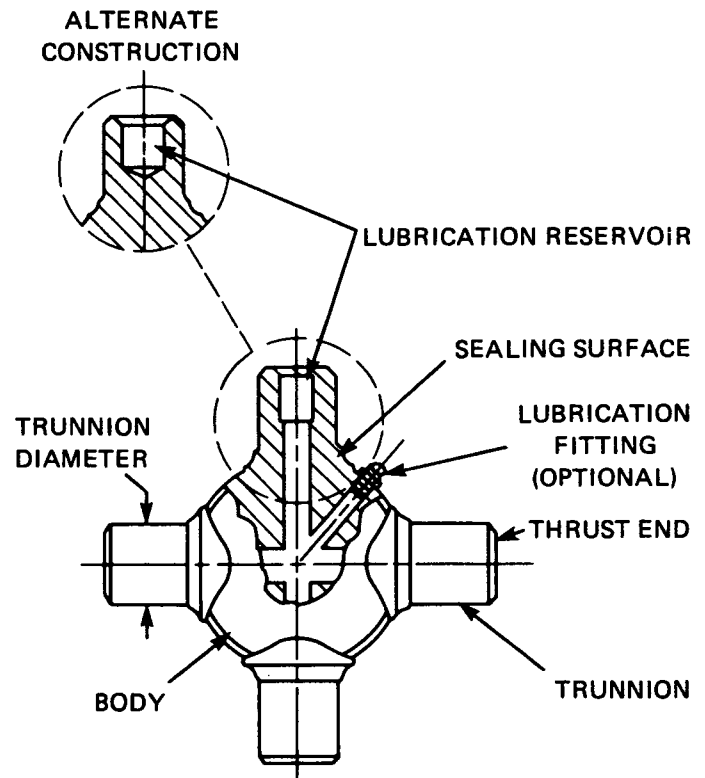
FIG. 10—CROSS
