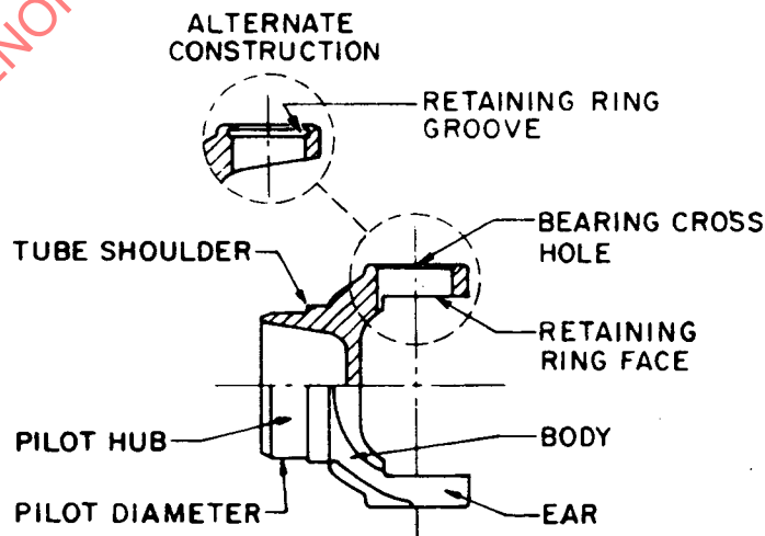
FIG. 3—TUBE OR WELD YOKE
