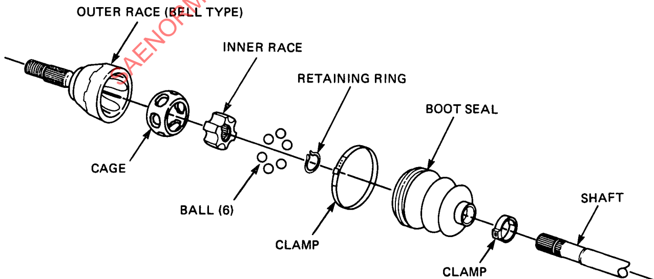
FIG. 17—RZEPPA UNIVERSAL JOINT
