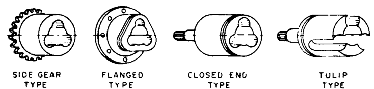
FIG. 14—TYPICAL TRIPOT OR TRIPOD JOINT HOUSING CONSTRUCTIONS
