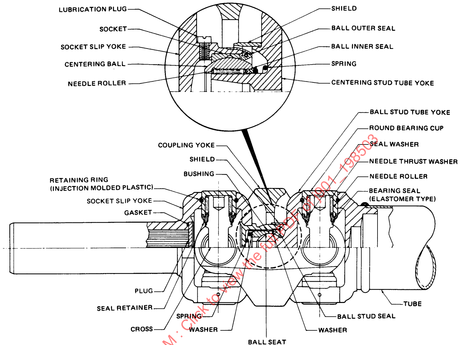
FIG. 11—DOUBLE CARDAN UNIVERSAL JOINT
