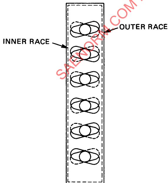
FIG. 19—DEVELOPMENT VIEW OF CROSS GROOVE JOINT ILLUSTRATING RELATIONSHIP OF OUTER AND INNER RACE BALL GROOVES AND POSITIONING OF BALLS
