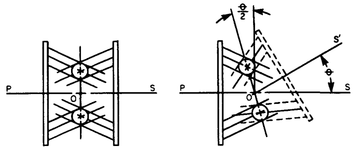
FIG. 20—DIAGRAM ILLUSTRATING POSITIONING OF BALLS IN CROSS GROOVE JOINT BISECTING ANGLE PLANE
