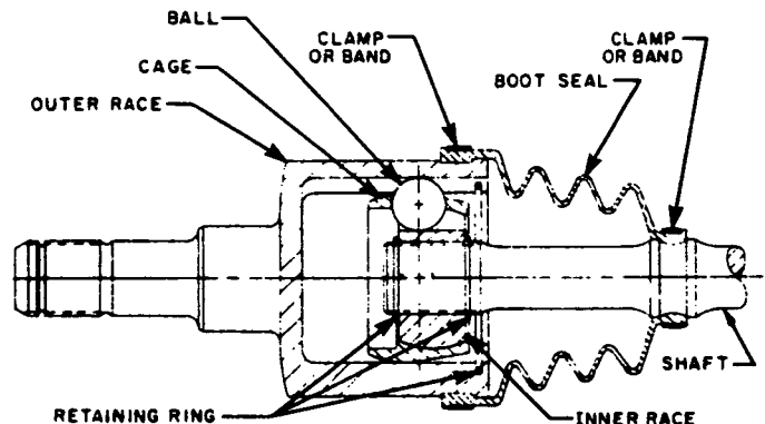
FIG. 22—DOUBLE OFFSET OR DO UNIVERSAL JOINT (END MOTION TYPE)
