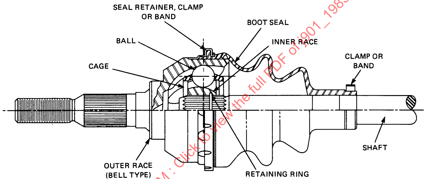
FIG. 16—RZEPPA UNIVERSAL JOINT
