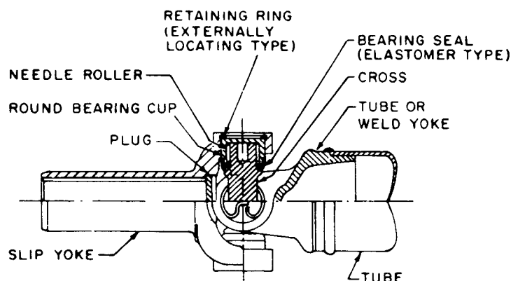
FIG. 1—CARDAN UNIVERSAL JOINT
