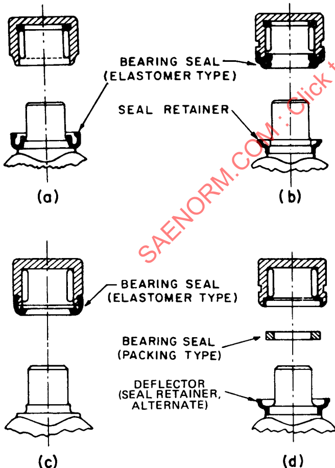
FIG. 9—BEARING SEAL TYPES
