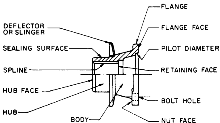
FIG. 7—COMPANION FLANGE
