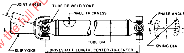
(a) TWO-JOINT OUTBOARD SLIP DRIVESHAFT
