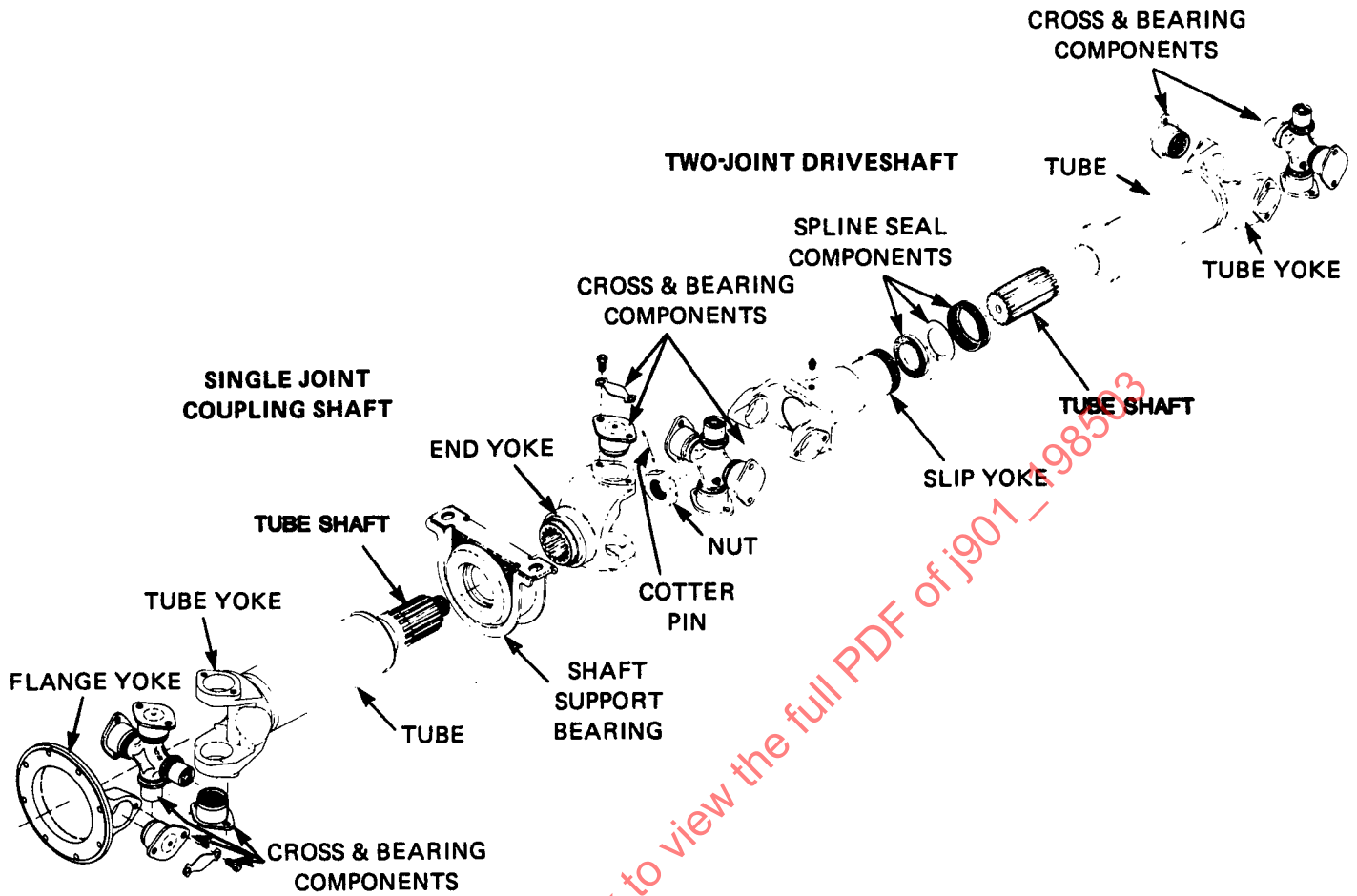
FIG. 28—TYPICAL TWO-PIECE HEAVY-DUTY TRUCK DRIVELINE
