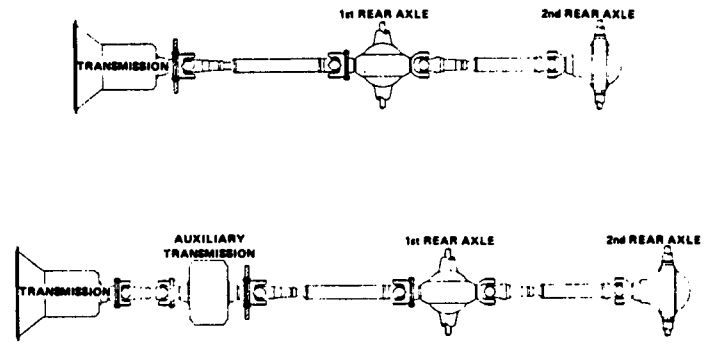
FIG. 32—TYPICAL 6 X 4 TRUCK DRIVELINE ARRANGEMENTS
