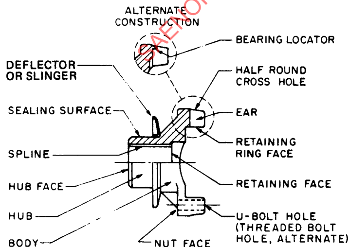
FIG. 5—END YOKE (ROUND BEARING TYPE)
