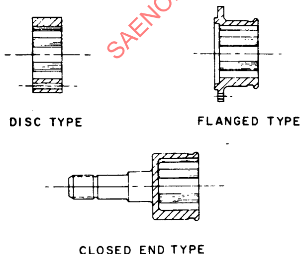
FIG. 24—TYPICAL DOUBLE OFFSET JOINT OUTER RACE CONSTRUCTIONS
