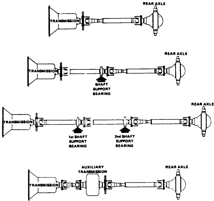
FIG. 30—TYPICAL 4 X 2 AND 6 X 2 TRUCK DRIVELINE ARRANGEMENTS
