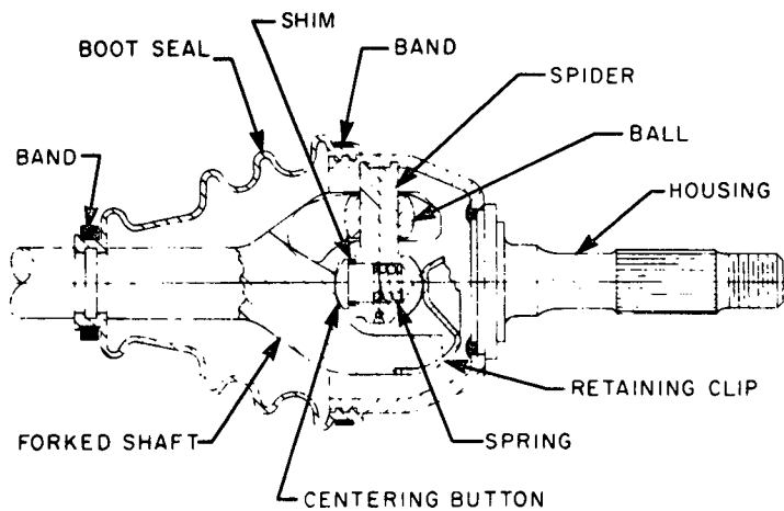
FIG. 15—TRIPOT OR TRIPOD UNIVERSAL JOINT (FIXED CENTER TYPE)
