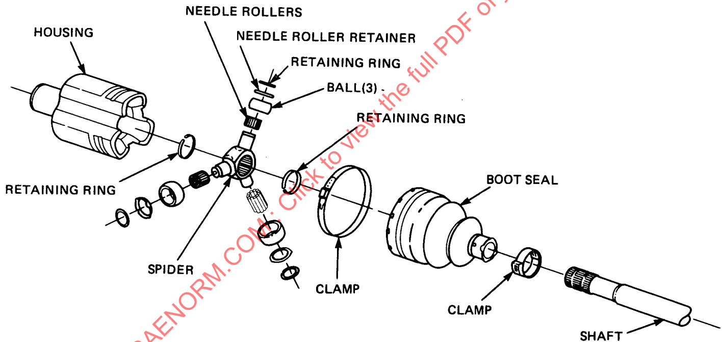
FIG. 13—TRIPOT OR TRIPOD UNIVERSAL JOINT (END MOTION TYPE)
