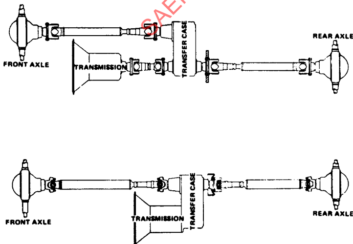
FIG. 31—TYPICAL 4 X 4 TRUCK DRIVELINE ARRANGEMENTS
