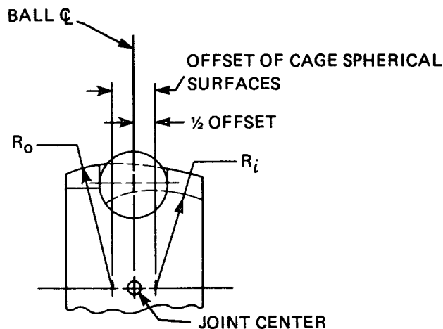
FIG. 23—DIAGRAM ILLUSTRATING OFFSET RELATIONSHIP OF DOUBLE OFFSET CAGE SPHERICAL SURFACES
