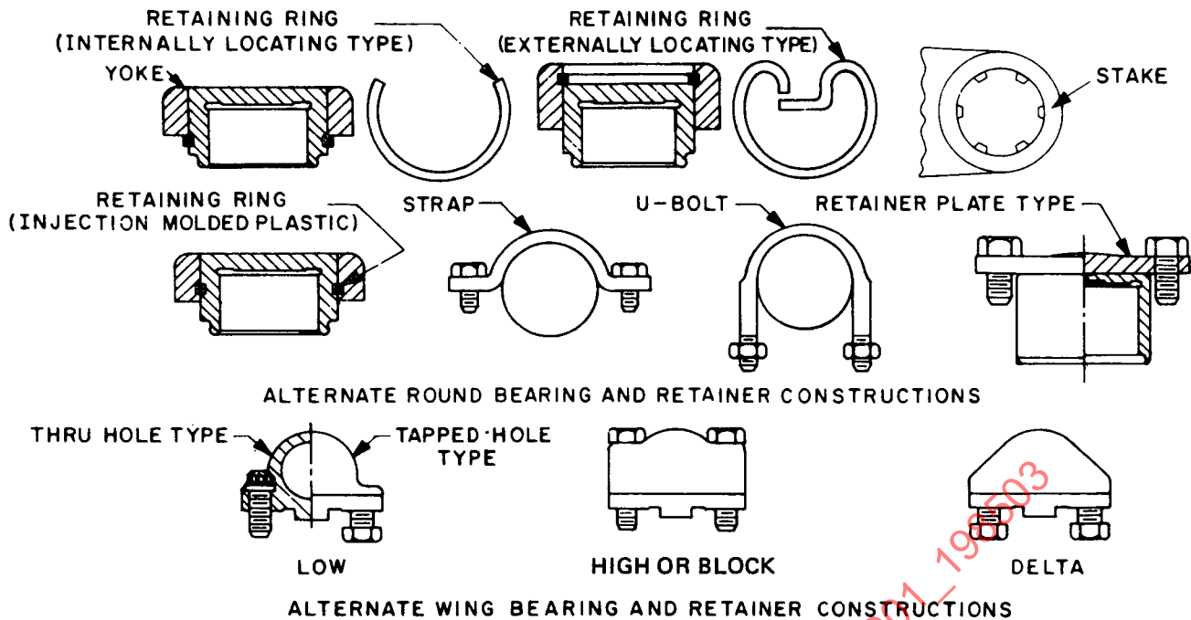
FIG. 8—BEARING AND RETAINER TYPES
