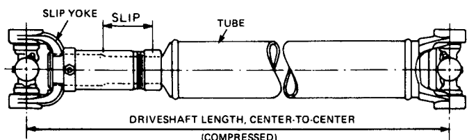
(b) TWO-JOINT INBOARD SLIP DRIVESHAFT
