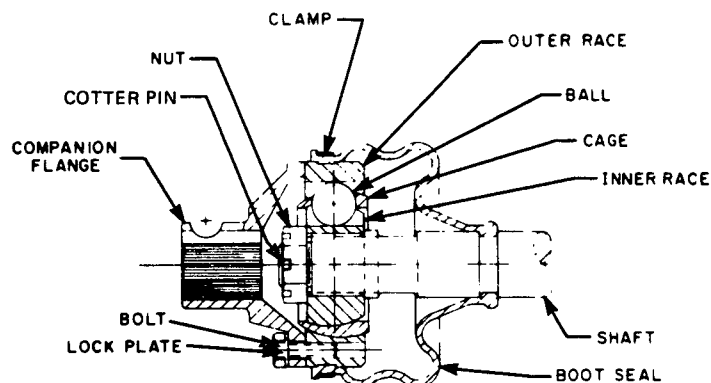
FIG. 25—DOUBLE OFFSET OR DO UNIVERSAL JOINT (FIXED CENTER TYPE)—STEERING SHAFT DESIGN ILLUSTRATED
