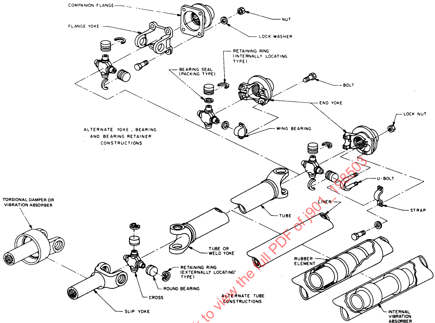
FIG. 27—TYPICAL TWO-JOINT OUTBOARD SLIP DRIVESHAFT
