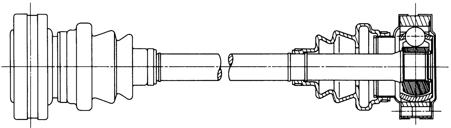
FIG. 35—TYPICAL REAR WHEEL DRIVE HALFSHAFT WITH END MOTION UNIVERSAL JOINTS (CROSS GROOVE TYPE SHOWN)
