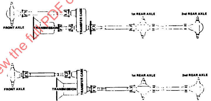
FIG. 33—TYPICAL 6 X 6 TRUCK DRIVELINE ARRANGEMENTS
