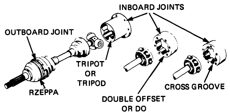
FIG. 34—TYPICAL FRONT WHEEL DRIVE HALFSHAFT WITH ALTERNATE INBOARD END MOTION UNIVERSAL JOINTS
