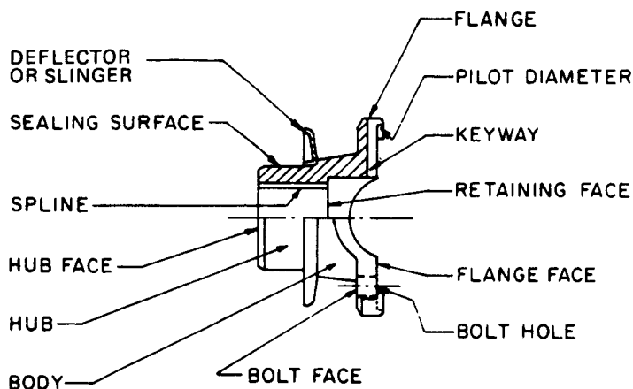
FIG. 4—END YOKE (WING BEARING TYPE)
