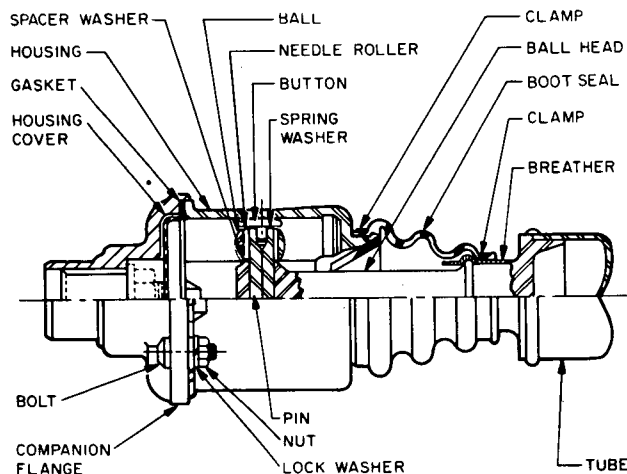
FIG. 3—BALL AND TRUNNION UNIVERSAL JOINT
