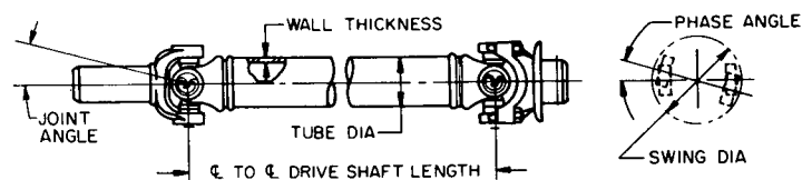
FIG. 1 — ONE-PIECE TUBULAR DRIVE SHAFT TERMINOLOGY
