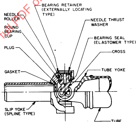
FIG. 2—CARDAN UNIVERSAL JOINT
