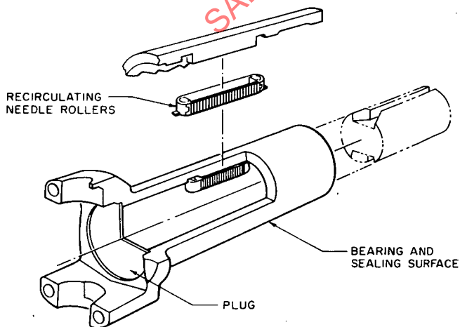
FIG. 13—SLIP YOKE (RECIRCULATING NEEDLE ROLLER TYPE)
