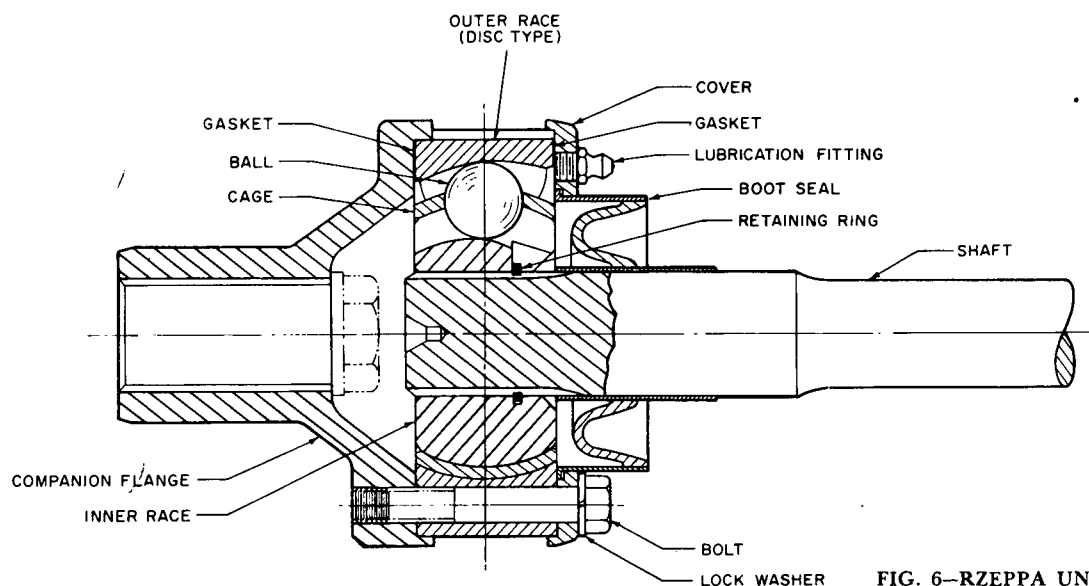
FIG. 6—RZEPPA UNIVERSAL JOINT (DISC TYPE)
