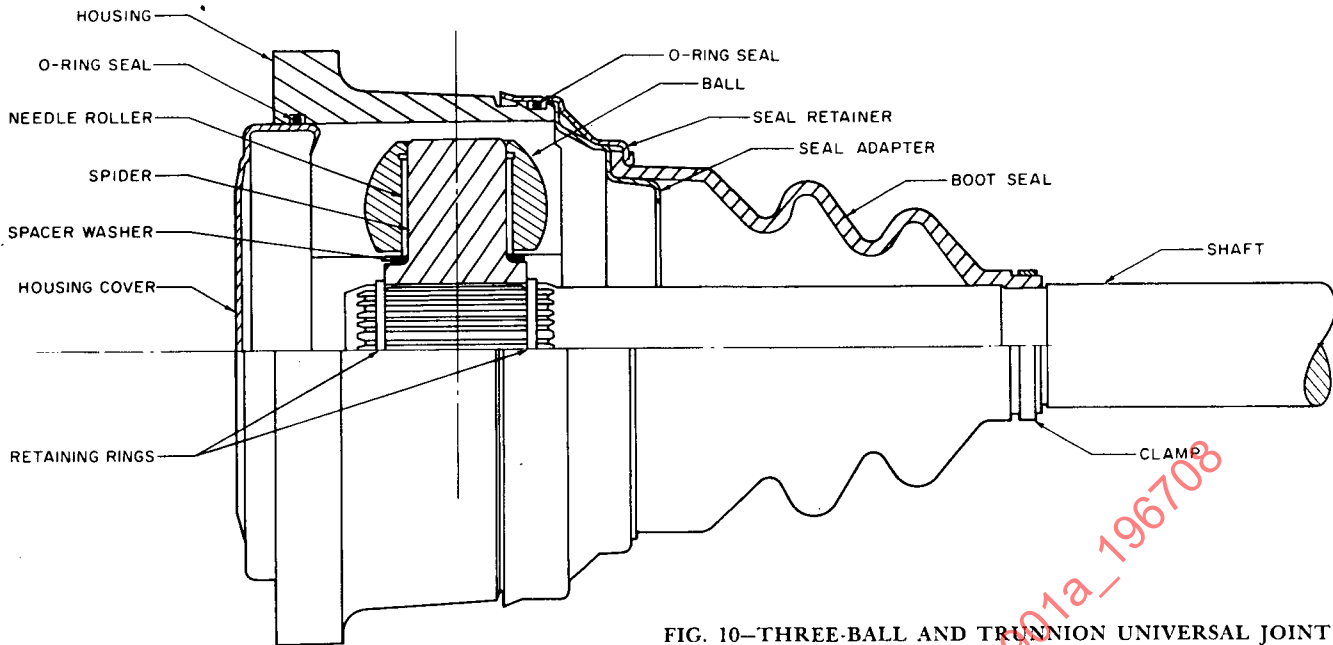
FIG. 10—THREE-BALL AND TRUNNION UNIVERSAL JOINT
