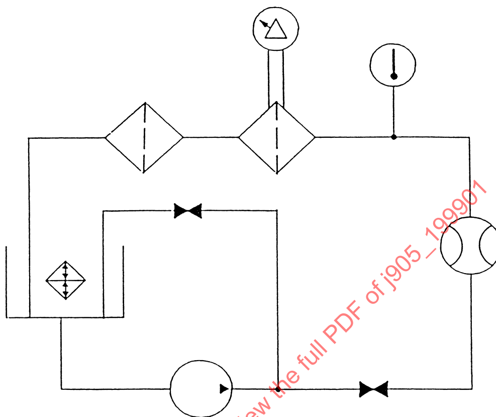
FIGURE 6—MEDIA MIGRATION TEST STAND
