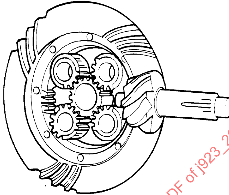
FIGURE 4A—DOUBLE-REDUCTION PLANETARY DIFFERENTIAL GEARING
