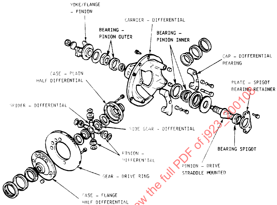
FIGURE 3—PINION MOUNTING OPTIONS
