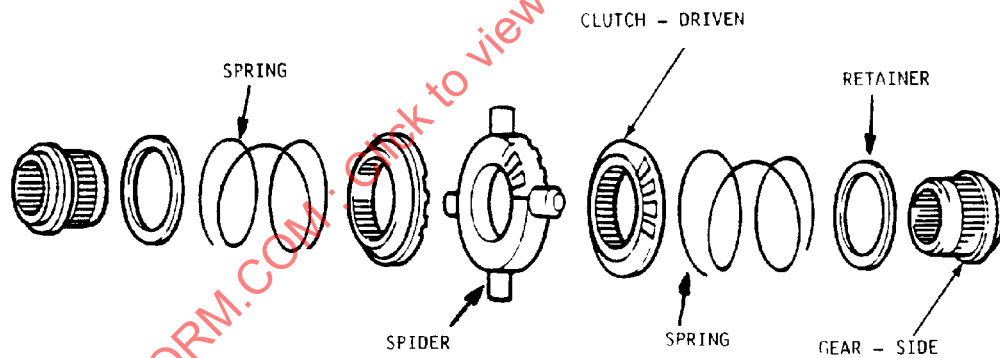
FIGURE 8B—AUTOMATIC POSITIVE LOCKING DIFFERENTIAL
