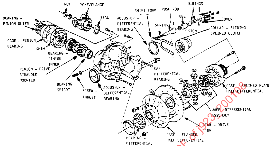
FIGURE 8C—POSITIVE DIFFERENTIAL LOCK—SLIDING SPLINED COLLAR CONSTRUCTION
