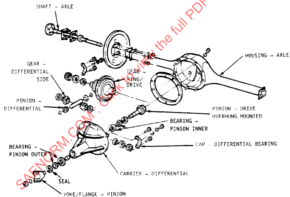
FIGURE 2—SEPARABLE CARRIER-HOUSING CONSTRUCTION
