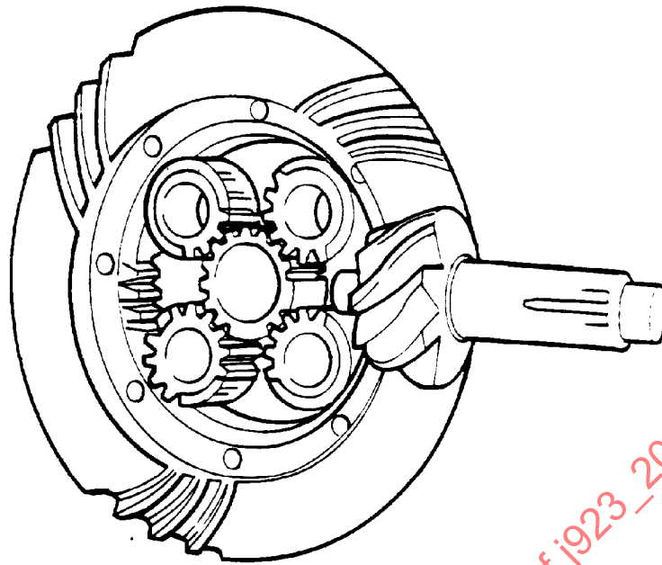
FIGURE 4A—DOUBLE-REDUCTION PLANETARY DIFFERENTIAL GEARING
