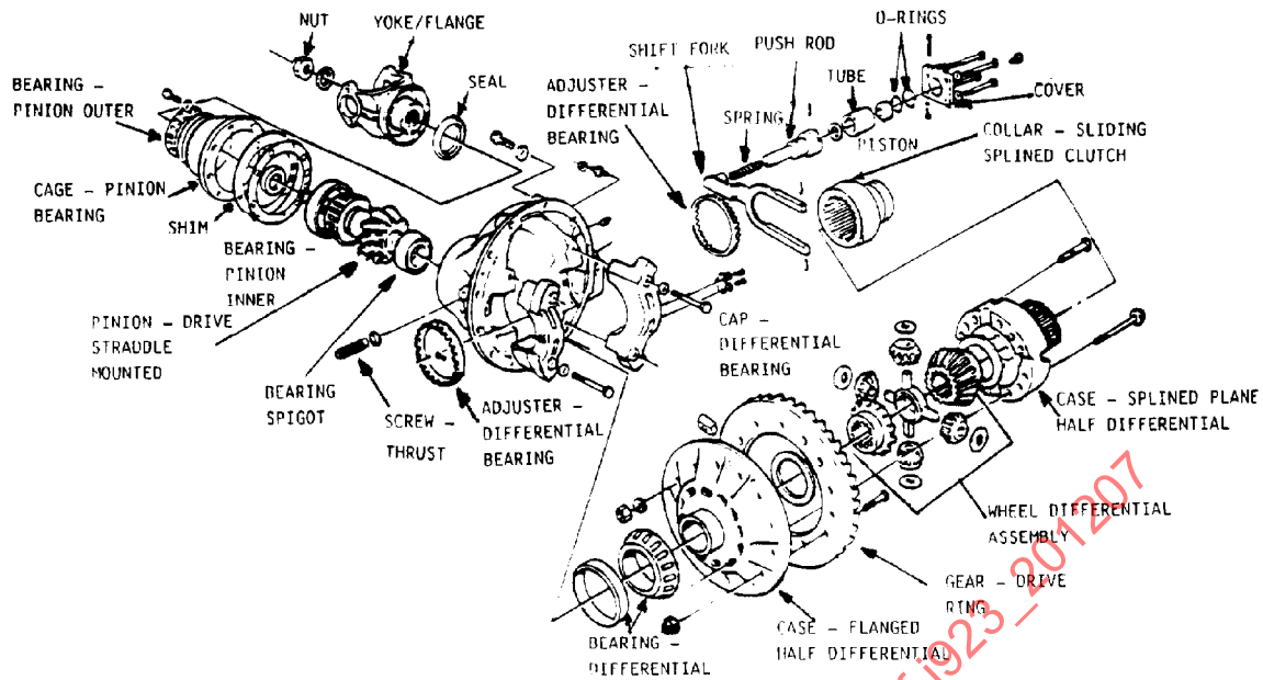
FIGURE 8C—POSITIVE DIFFERENTIAL LOCK—SLIDING SPLINED COLLAR CONSTRUCTION
