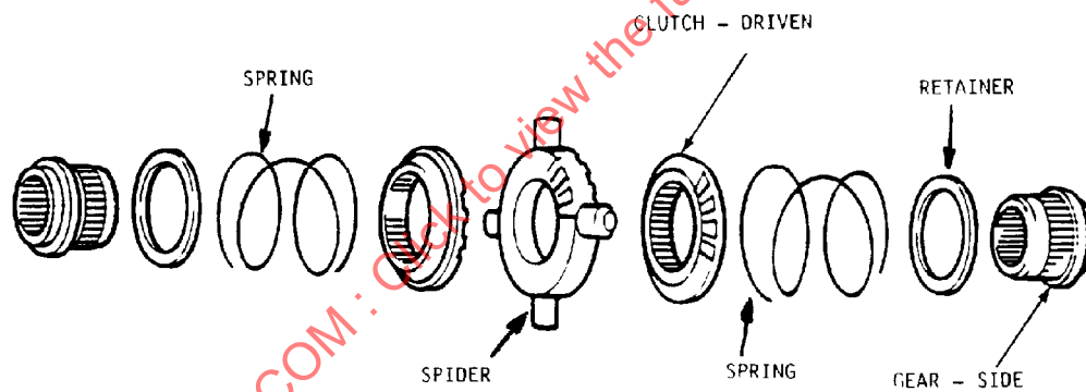
FIGURE 8B—AUTOMATIC POSITIVE LOCKING DIFFERENTIAL
