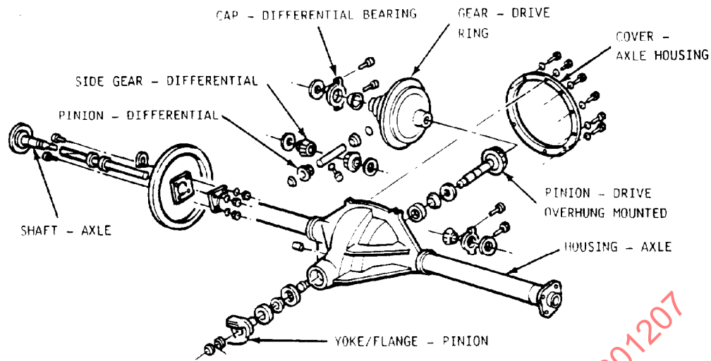
FIGURE 1—UNITIZED CARRIER-HOUSING CONSTRUCTION
