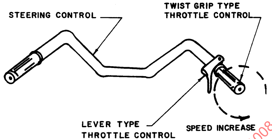
FIGURE 1 - THROTTLE CONTROL
