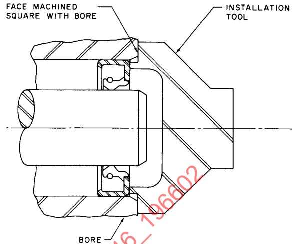
FIG. 3—THROUGH BORE: INSTALLATION TOOL BOTTOMS ON MACHINED BORE FACE
