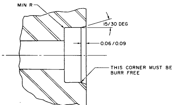
FIG. 2—RECOMMENDED BORE LEAD CORNER
