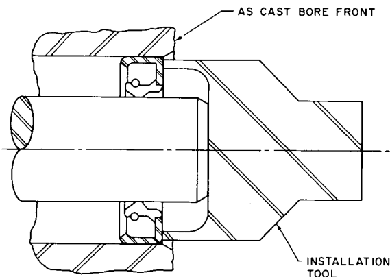
FIG. 5—THROUGH BORE: INSTALLATION TOOL BOTTOMS ON SHAFT
