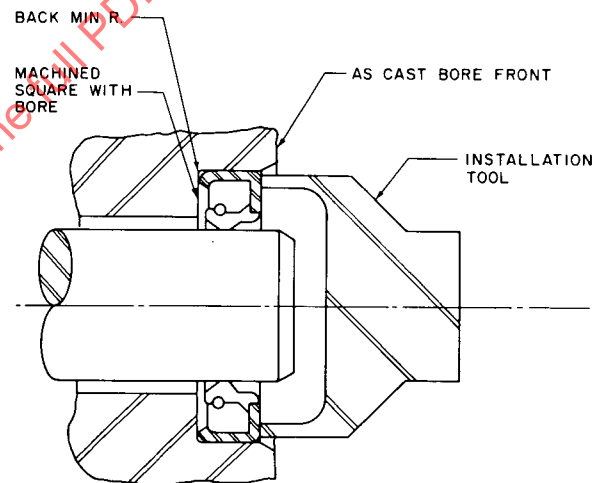
FIG. 4—BOTTOM BORE: SEAL BOTTOMS ON MACHINE BORE SHOULDER
