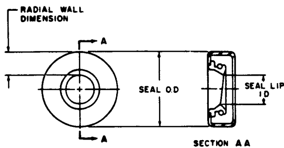
FIG. 13 - RADIAL WALL DIMENSION
