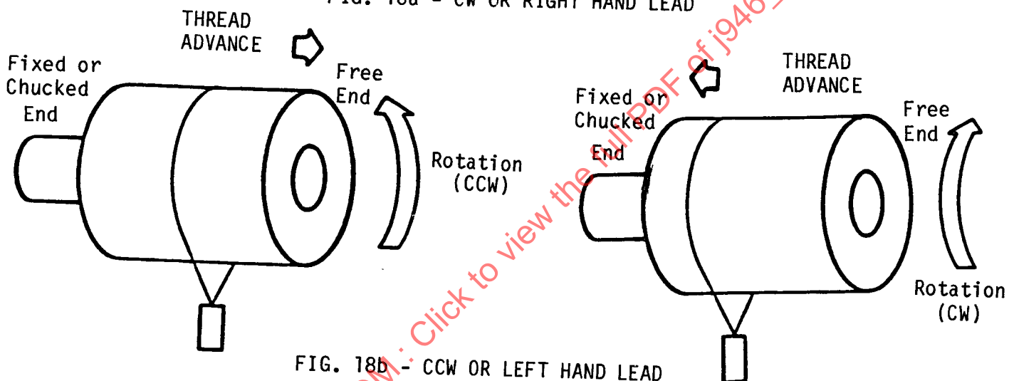
FIG. 18a - CW OR RIGHT HAND LEAD
