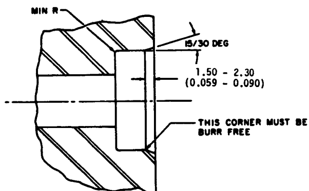
FIG. 6 - RECOMMENDED BORE LEAD CORNER
