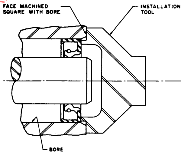
FIG. 7 - THROUGH BORE: INSTALLATION TOOL BOTTOMS ON MACHINED BORE FACE
