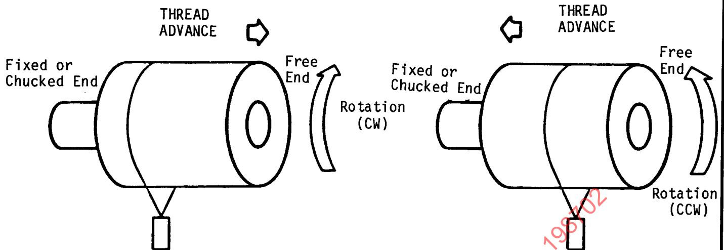
FIG. 18a - CW OR RIGHT HAND LEAD
