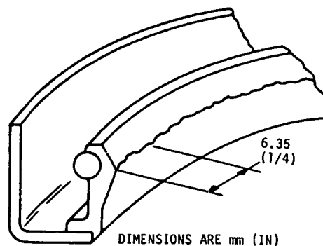
FIG. 15 - MEASUREMENT OF CONTACT LINE HEIGHT VARIATION
