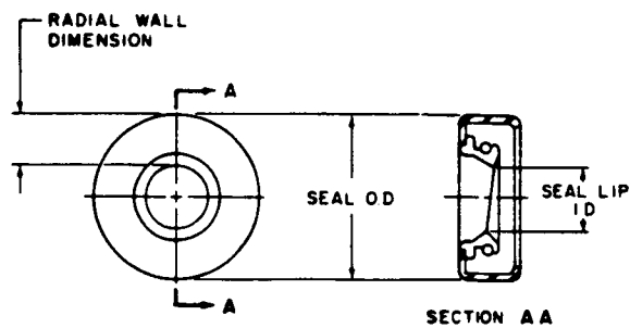
FIGURE 13 - Radial Wall Dimension
