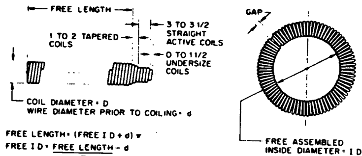
FIGURE 10 - Spring Nomenclature
