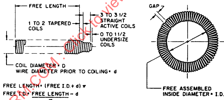
FIGURE 12—SPRING NOMENCLATURE
