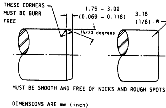
FIGURE 7—RECOMMENDED SHAFT LEAD CORNERS
