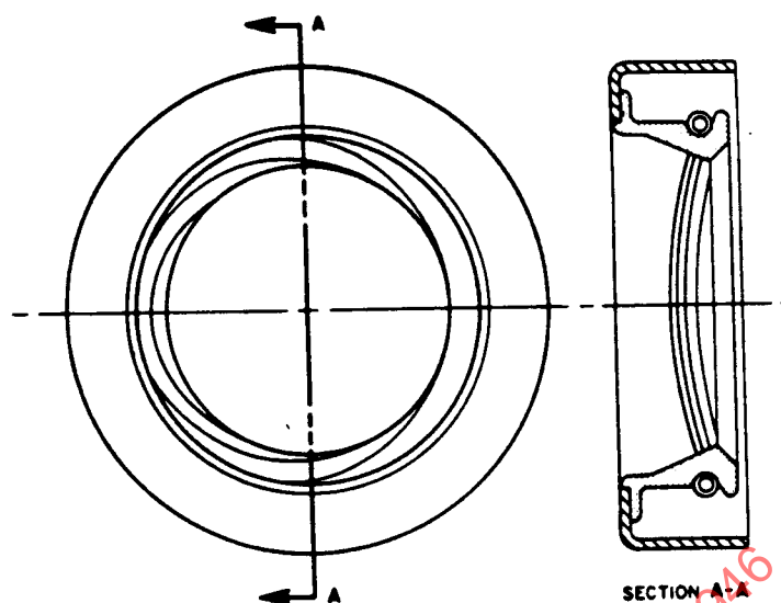
FIGURE 3—BIROTATIONAL ELASTOHYDRODYNAMIC SEAL: RIBS PROTRUDING IN OPPOSITE DIRECTIONS PRODUCE SEALING IRRESPECTIVE OF DIRECTION OF SHAFT ROTATION
