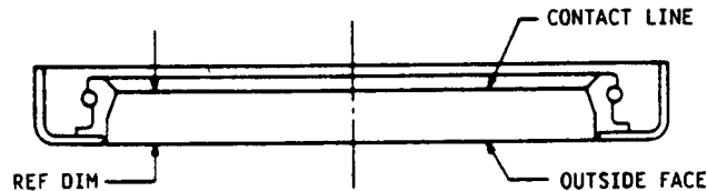
FIGURE 16—CONTACT LINE HEIGHT VARIATION
