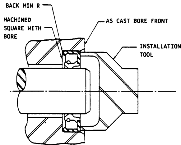
FIGURE 10—BOTTOM BORE: SEAL BOTTOMS ON MACHINE BORE SHOULDER CONFORMS WITH ISO 6194/3
