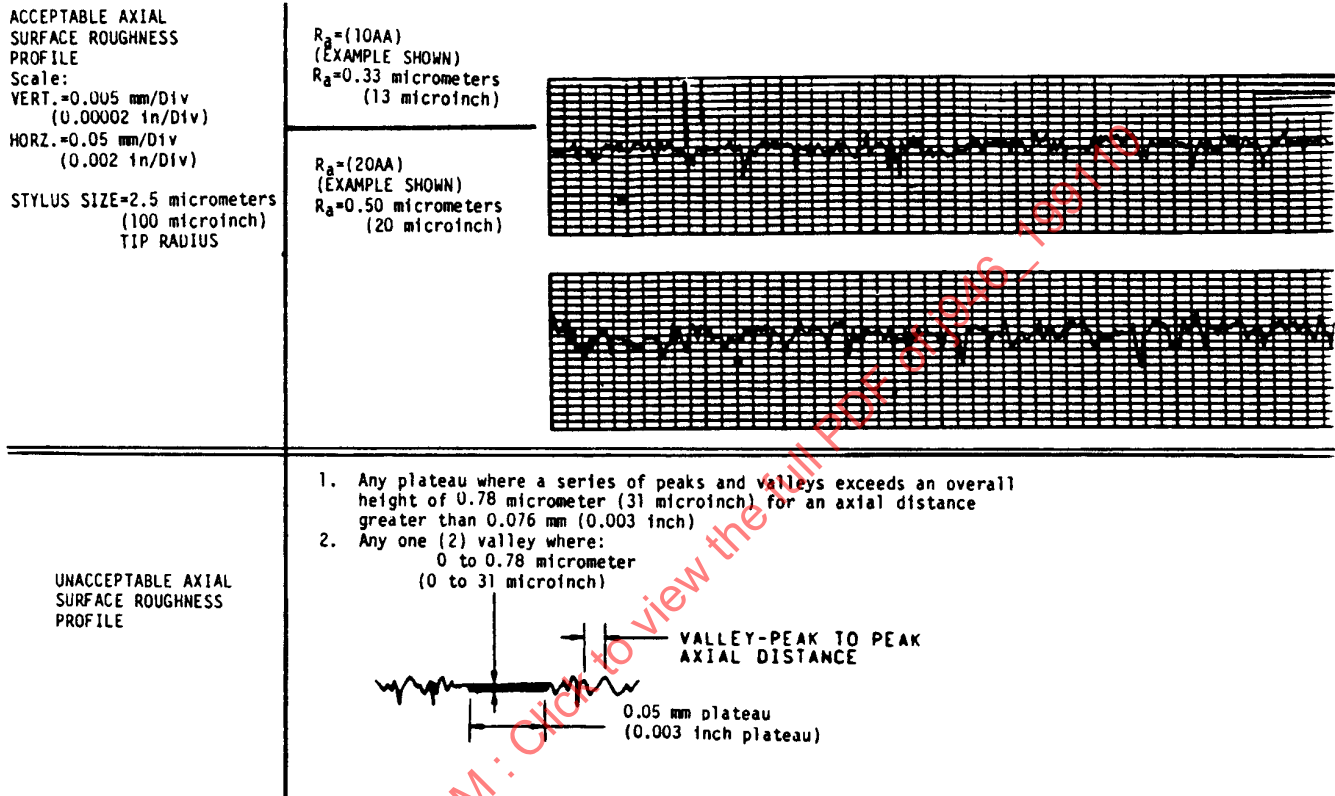
FIGURE 5—TYPICAL TRACES OF SHAFT SURFACE ROUGHNESS PROFILES
