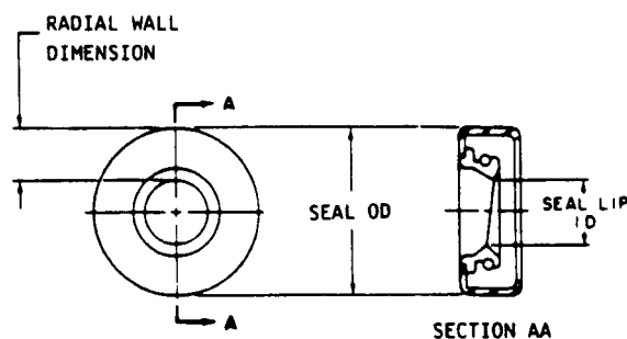
FIGURE 15—RADIAL WALL DIMENSION
