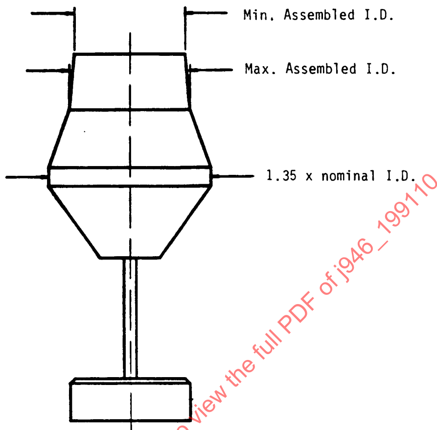
FIGURE 13—SPRING INSPECTION GAGE
