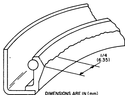
FIG. 12—MEASUREMENT OF CONTACT LINE HEIGHT VARIATION
