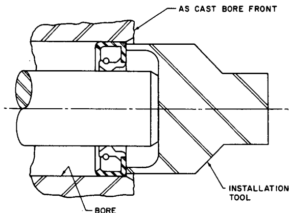
FIG. 9—THROUGH BORE: INSTALLATION TOOL BOTTOMS ON SHAFT
