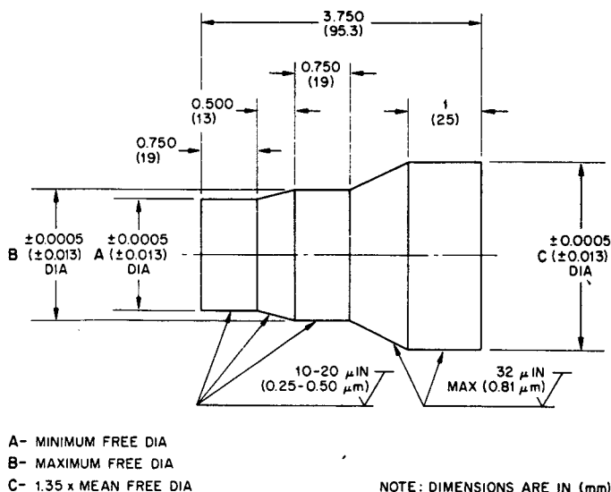
FIG. 15—SPRING INSPECTION MANDREL
