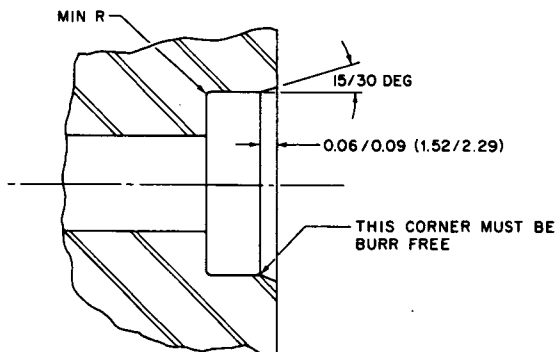
FIG. 5—RECOMMENDED SHAFT LEAD CORNERS
