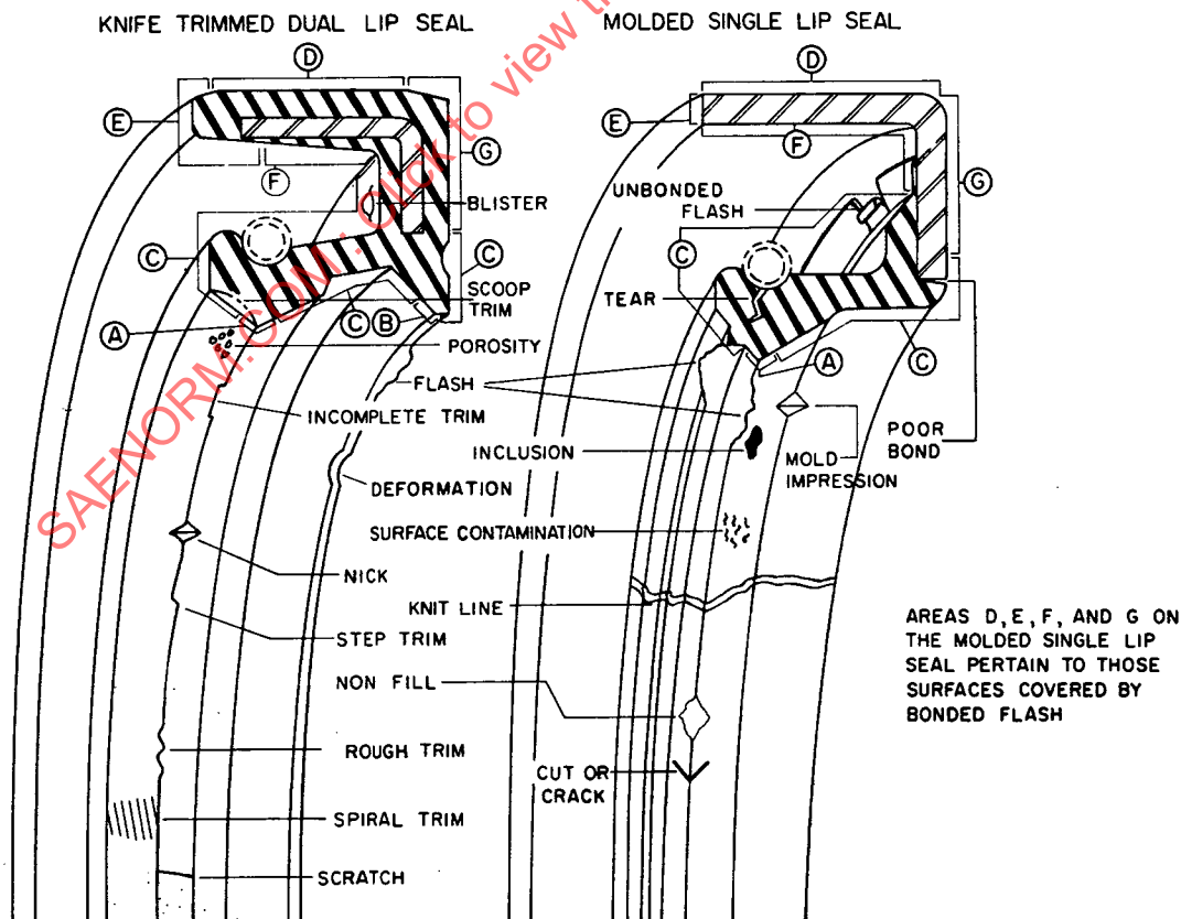
FIG. 18—VISUAL ELASTOMER VARIATIONS
