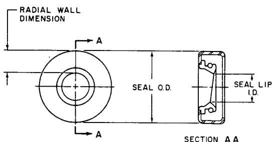
FIG. 10—RADIAL WALL DIMENSION
