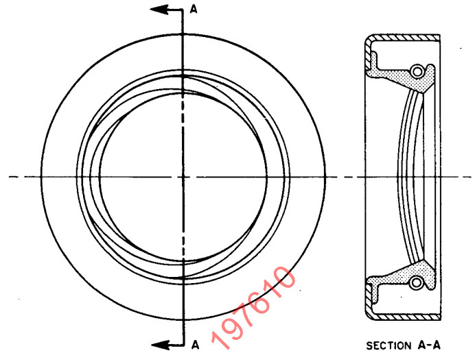
FIG. 2—BIROTATIONAL ELASTOHYDRODYNAMIC SEAL: RIBS PROTRUDING IN OPPOSITE DIRECTIONS PRODUCE SEALING IRRESPECTIVE OF DIRECTION OF SHAFT ROTATION
