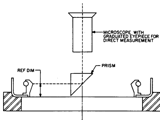
FIG. 12—MEASUREMENT OF CONTACT LINE HEIGHT VARIATION
