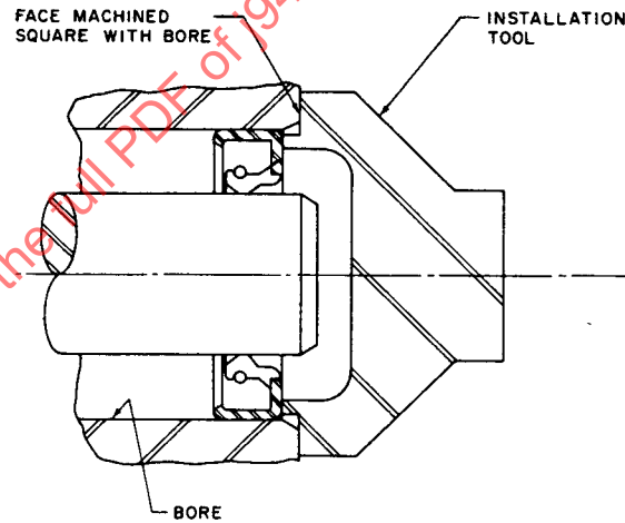
B. SEAL INSERTED BEYOND BORE FACE
