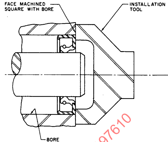
A. SEAL FLUSH WITH BORE FACE
