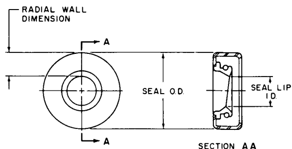
FIG. 10—RADIAL WALL DIMENSION
